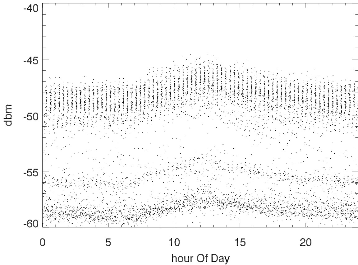
5020 power vs hour of day
