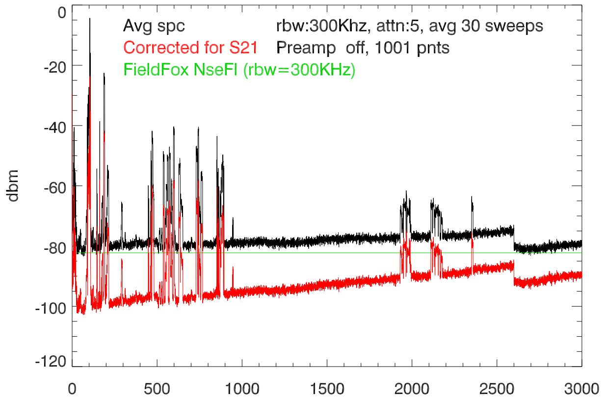
11may21 Input and S21 corrected spectra (FieldFox 9916A)
