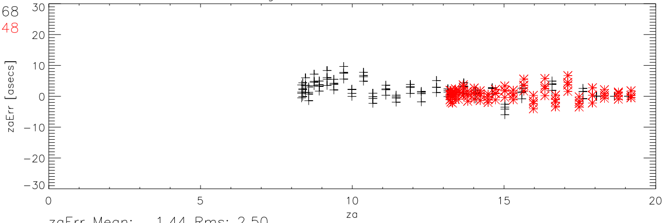
PntErrors cbandhi. aug13 data after ao19 removed. za error vs za
