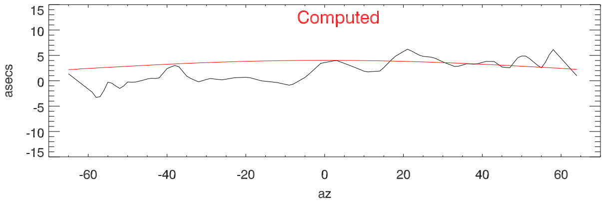
Za Err vs az for different offsets:(dh Td12= 0.500 In. dTheta Corner12: 26.33 Asecs)
