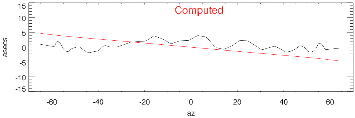
Az Err vs az for different offsets:(dh Td12= 0.500 In. dTheta Corner12: 26.33 Asecs)
