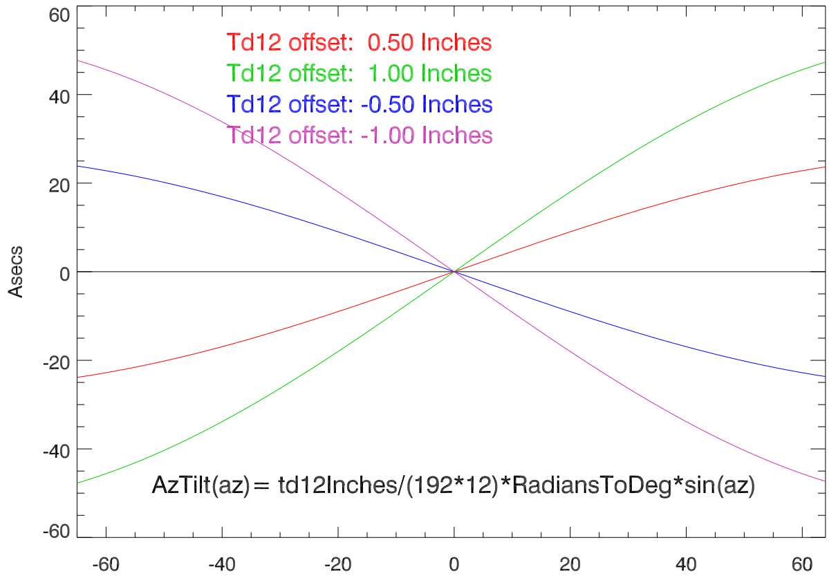
Platform Az tilt vs az for the various td12 offsets
