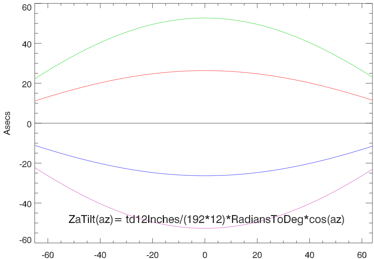
Platform Za tilt vs az for the various td12 offsets
