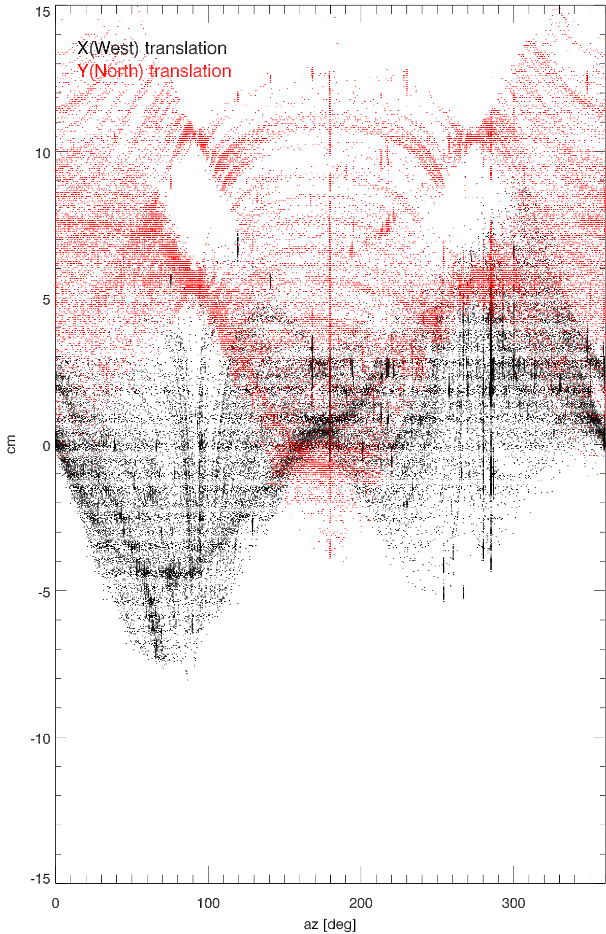
180101 to 180831 Platform translations x(west) and y(north) vs az. (all za)
