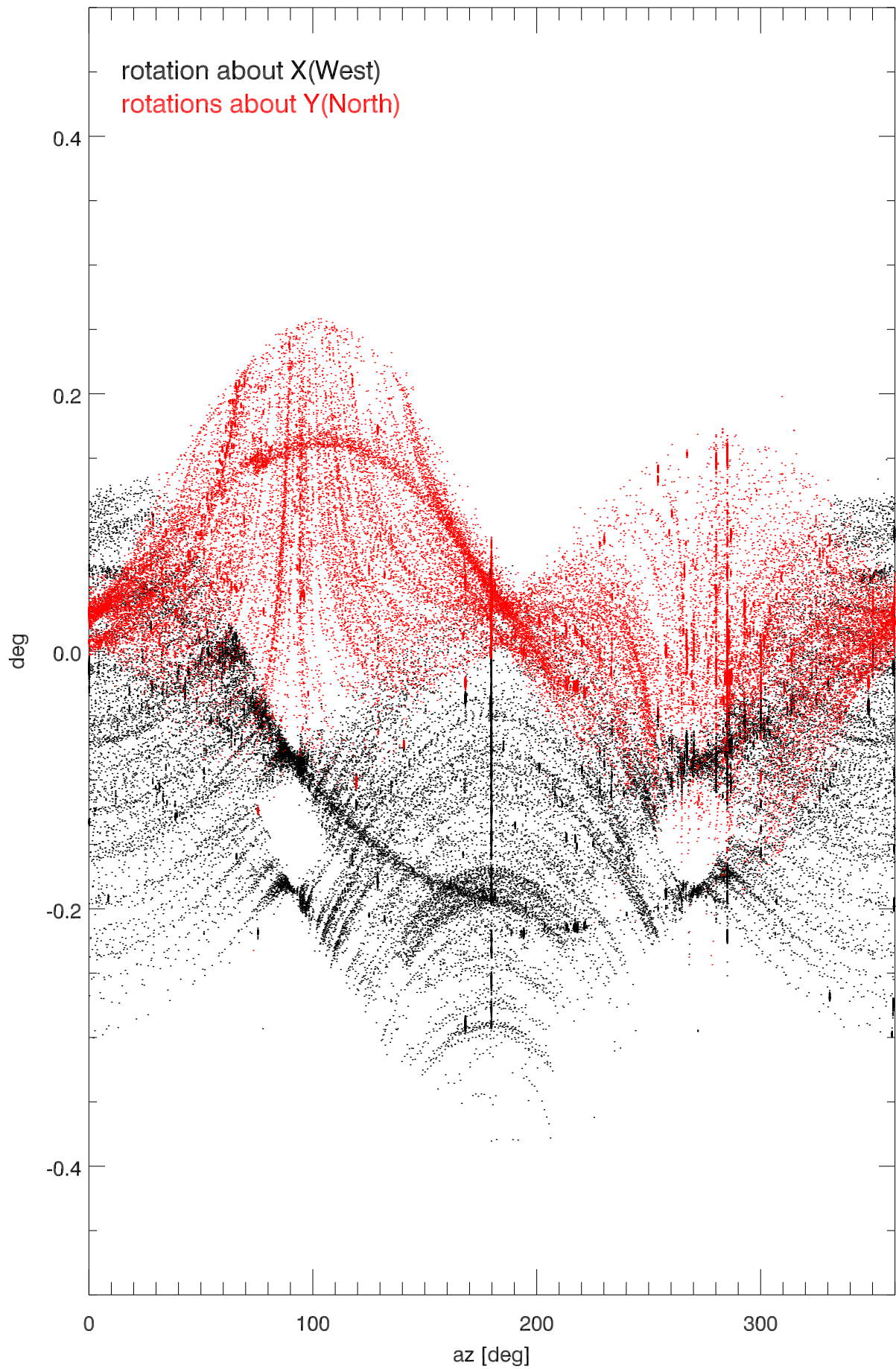
180101 to 180831 Platform rotations about x(west) and y(north) vs az. (all za)
