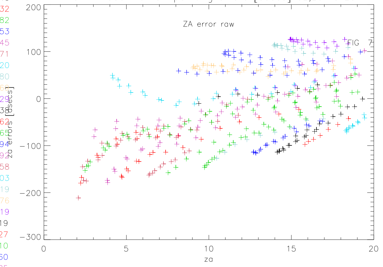
nov17model 19 raw pointing errors [asecs] az,za vs za
