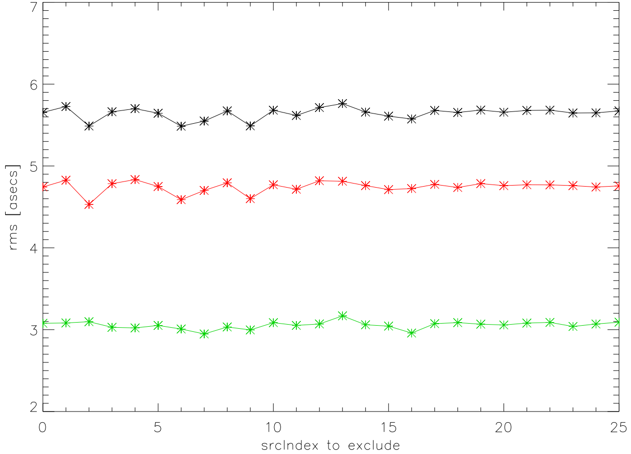
nov17 az,za,tot model rms excluding 1 src (with zaEncTable)
