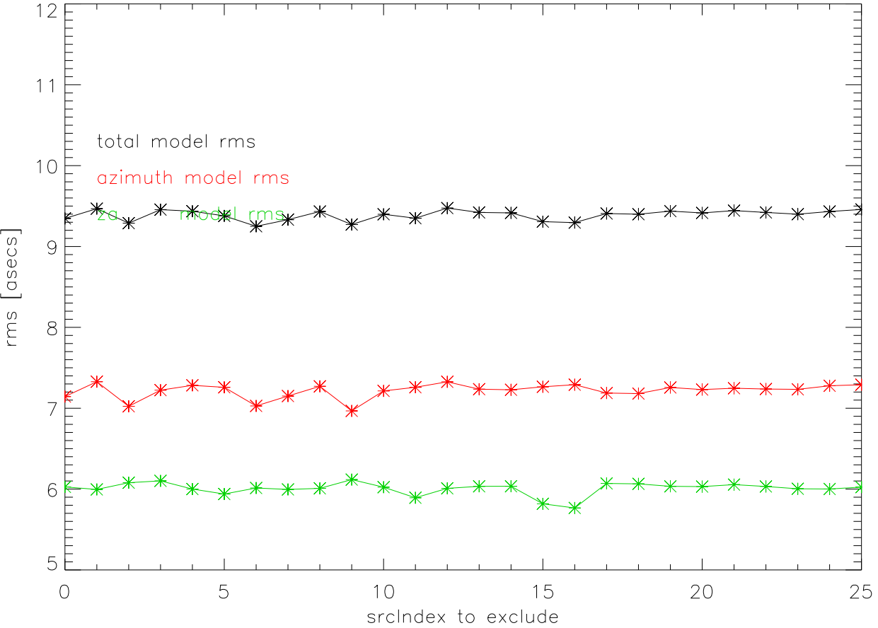
nov17 az,za,tot model rms excluding 1 src (noZaEncTable)
