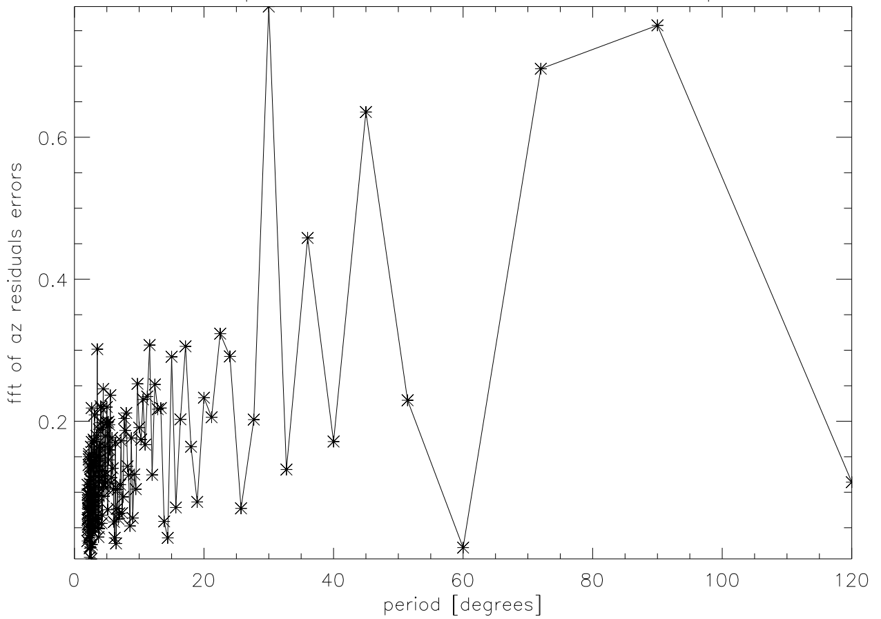
dec07 spectrum of az residual errors versus period
