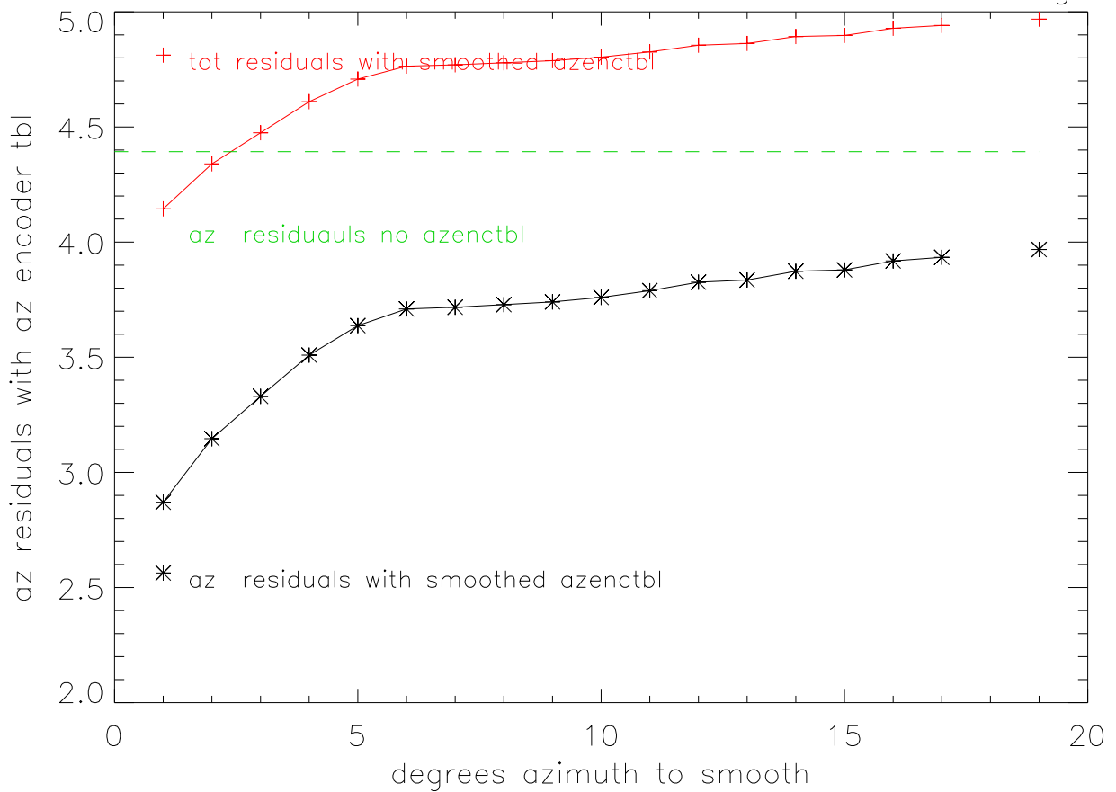
dec07 az residuals with encoder table versus smoothing length
