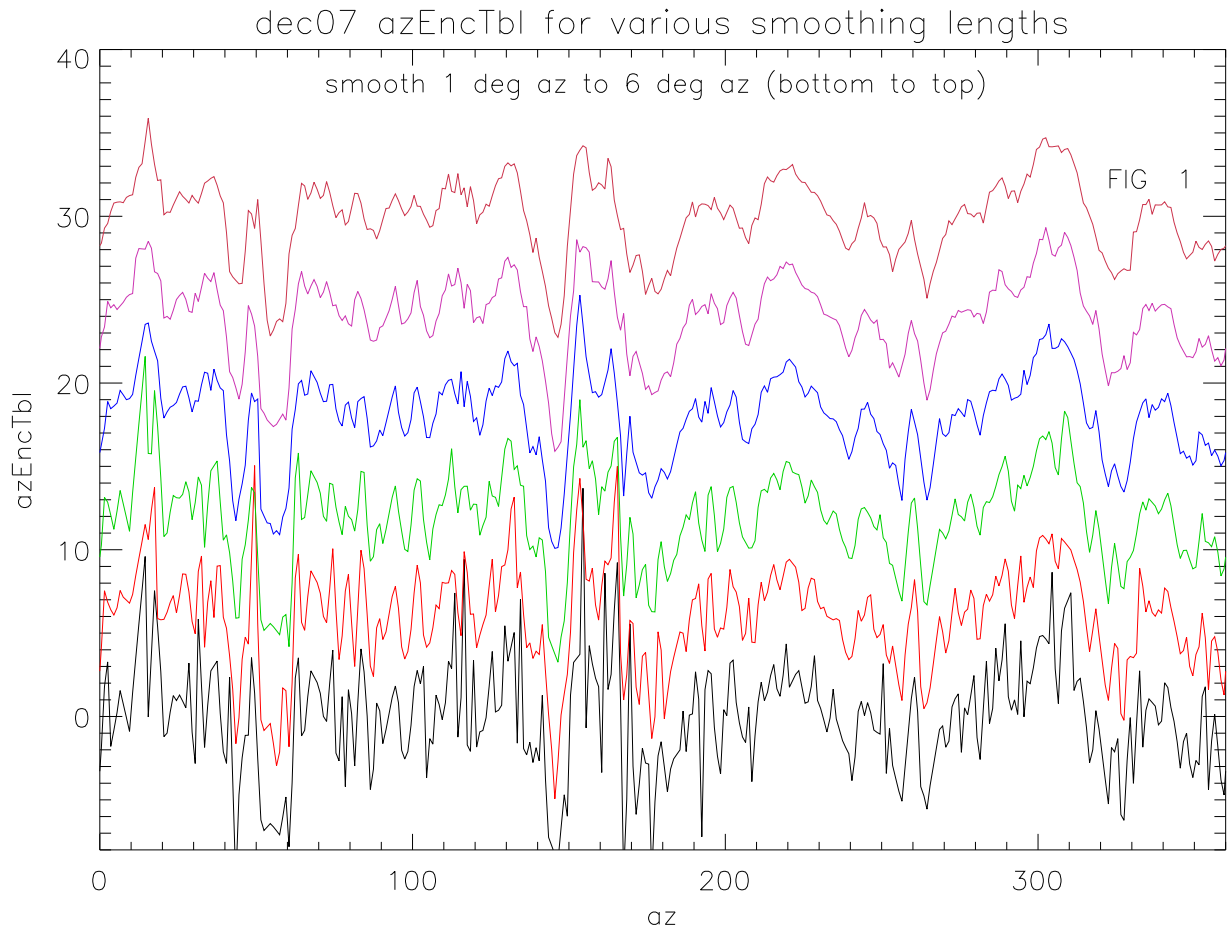
dec07 az residuals with encoder table versus smoothing length
