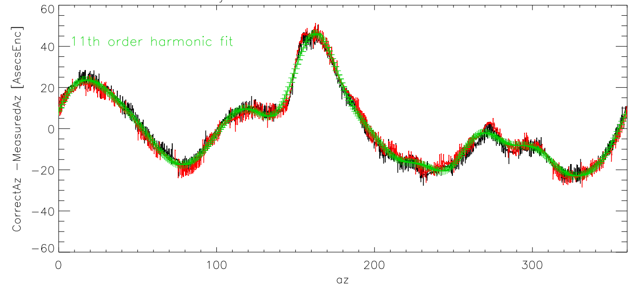
21jan00 azErr from runout versus az
