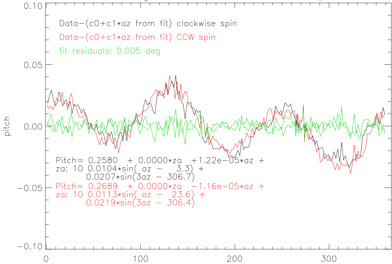
31mar07 4azsw @ 10deg za. tiltSensor frame PITCH - (c0+c1*az from fit)
