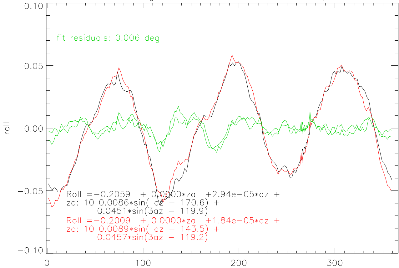
31mar07 4azsw @ 10deg za. tiltSensor frame Roll - (c0+c1*az from fit)
