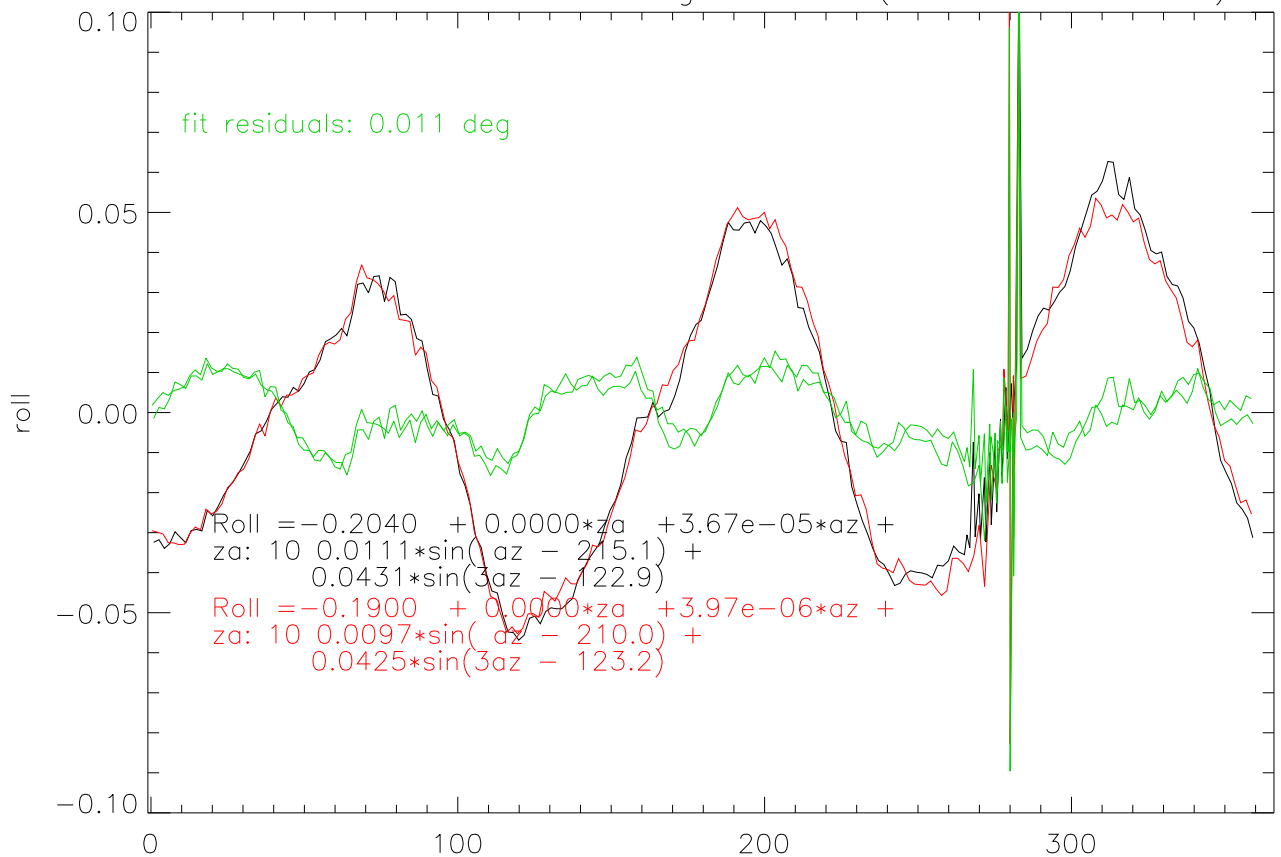
15feb12 tilt sensor az swings Roll - (c0+c1*az from fit)
