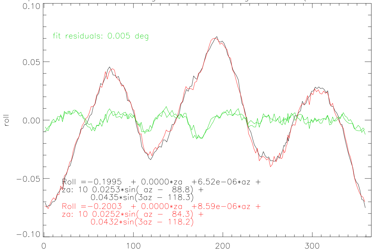
07apr07 tilt sensor az swings before td change Roll - (c0+c1*az from fit)
