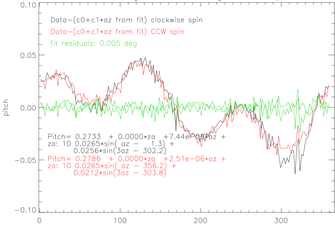
07apr07 tilt sensor az swings before td change PITCH - (c0+c1*az from fit)
