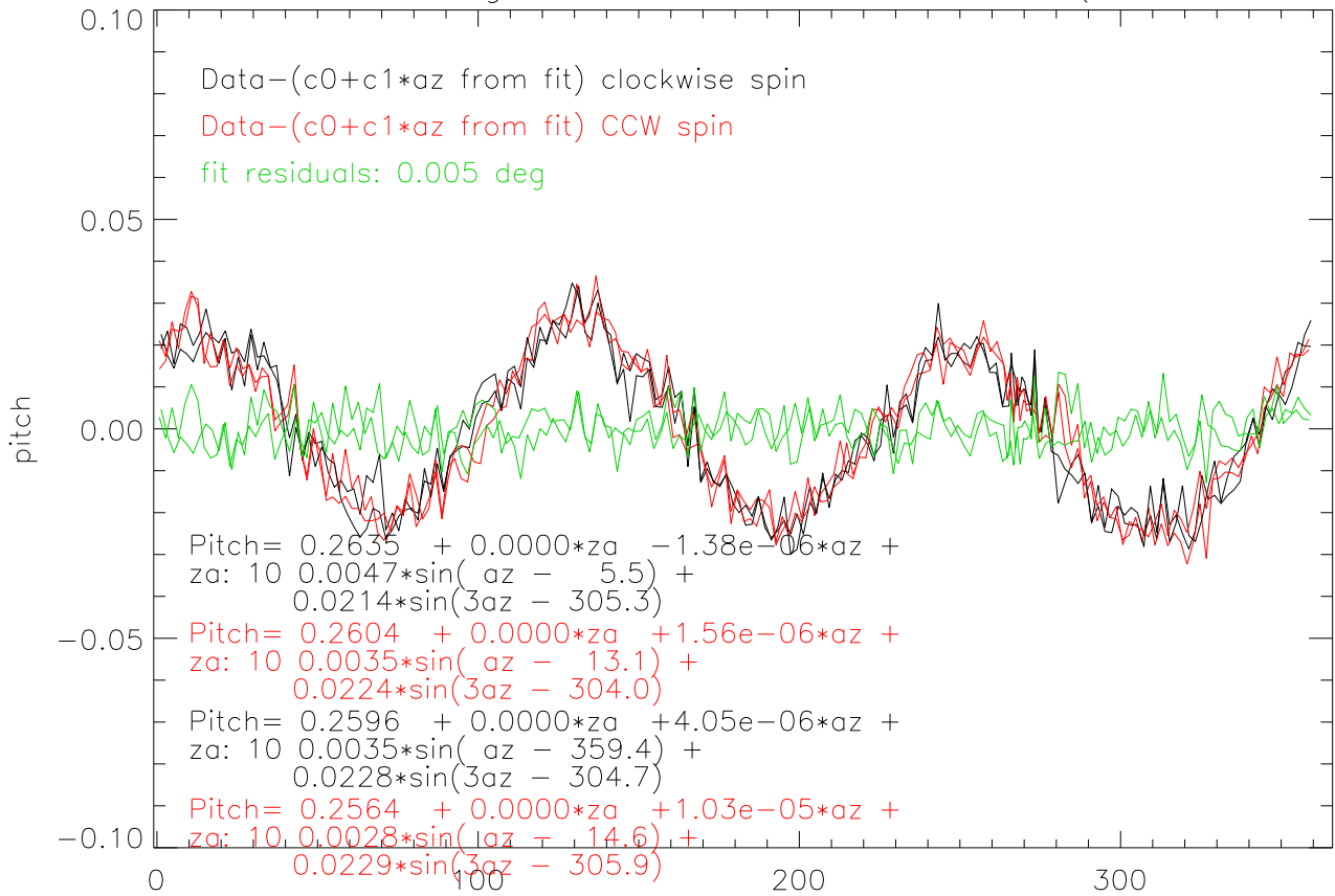
01dec06 4azsw @ 10deg za. tiltSensor frame PITCH - (c0+c1*az from fit)
