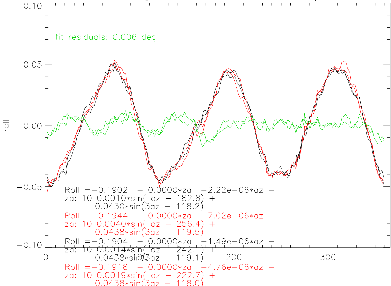
01dec06 4azsw @ 10deg za. tiltSensor frame Roll - (c0+c1*az from fit)
