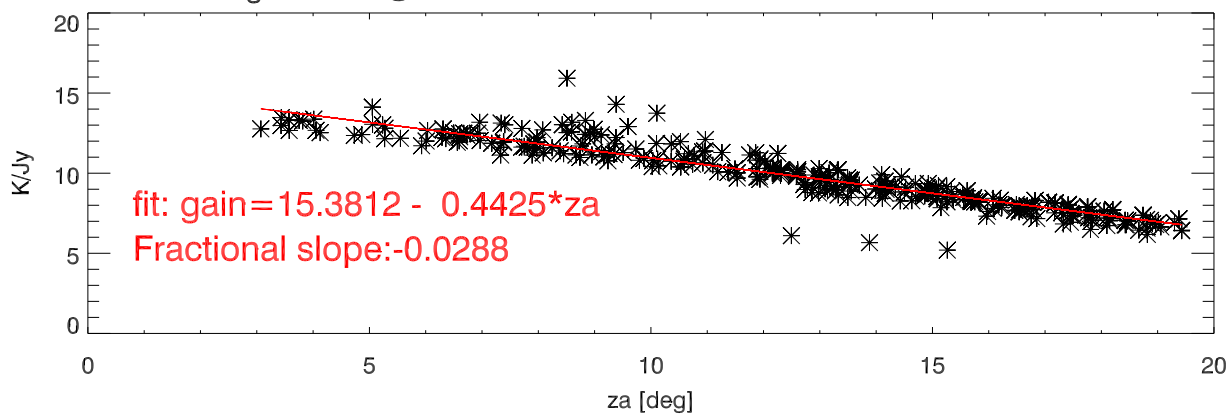
Ch gain vs za @ 430Mhz. 050301 to 120301. bandwidth:12.5000 Mhz
