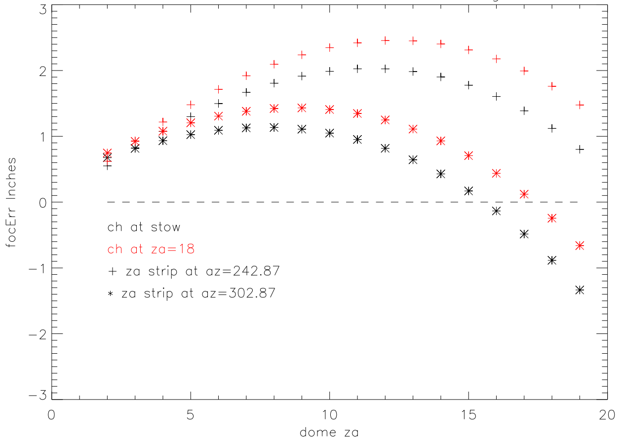
Focus error vs za. ch at stow and 18 deg za
