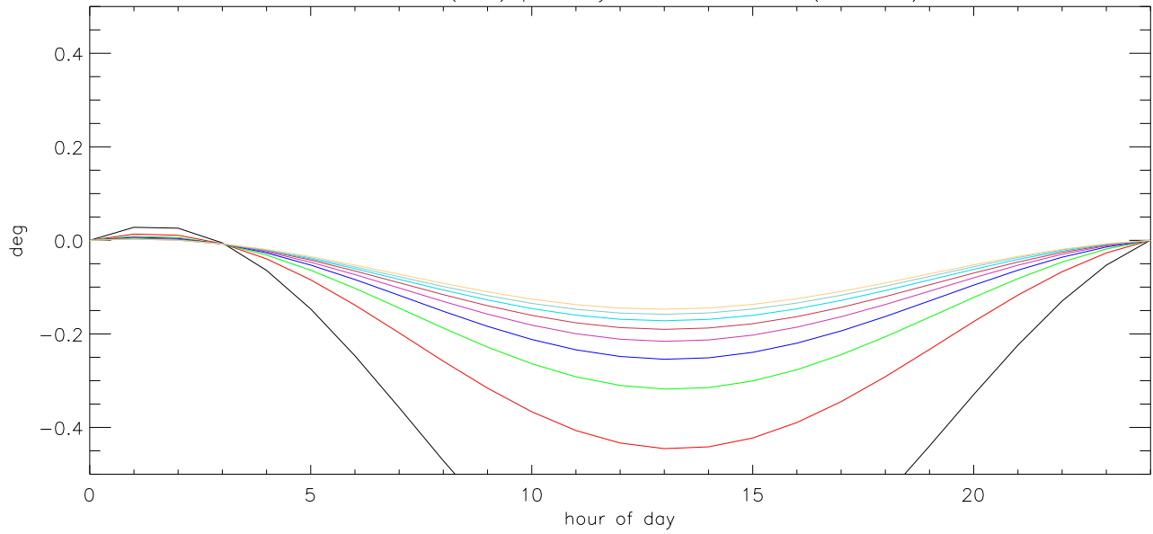
Az motion (on Sky) per day for J2000 drift (1mar06)
