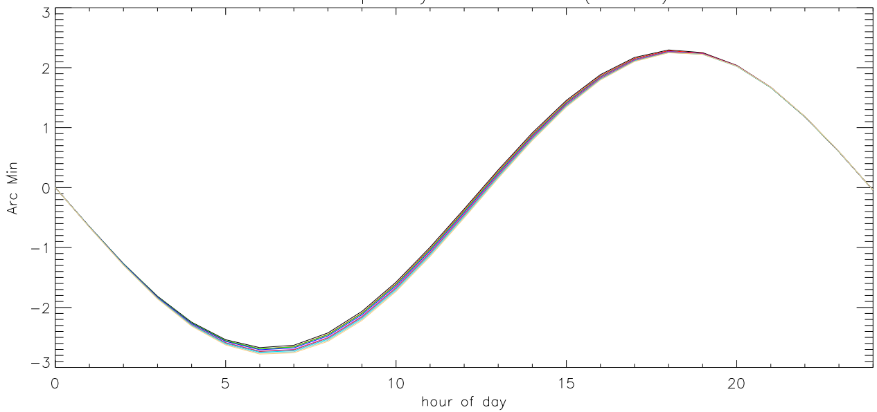
Za motion per day for J2000 drift (1mar07)
