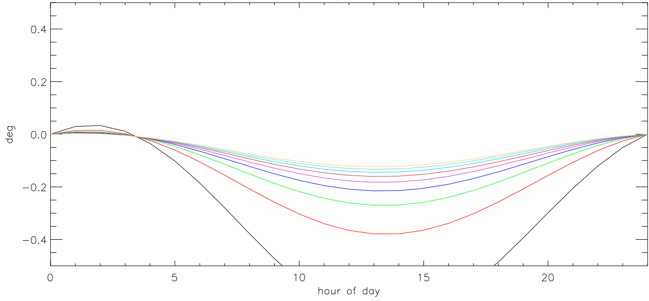
Az motion (on Sky) per day for J2000 drift (1mar05)
