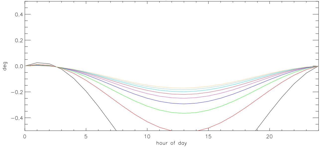
Az motion (on Sky) per day for J2000 drift (1mar07)
