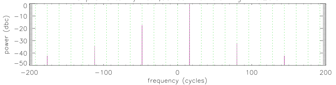
Clip sine to \pm 0.7 , dc:real= 0.10% img=-0.20%
