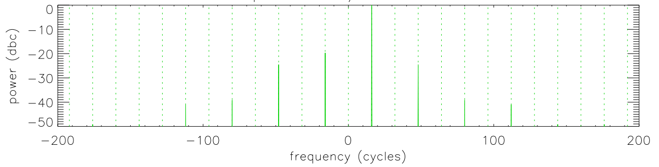
Clip sine to \pm 0.7 , dc:real= 0.10% img= 0.10%
