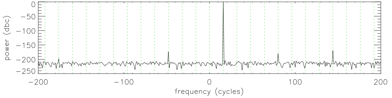
Clip sine to \pm 0.7 of max
