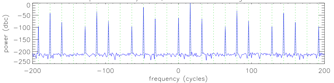
Clip sine to \pm 0.7 , dc:real= 0.10% img=-0.20%
