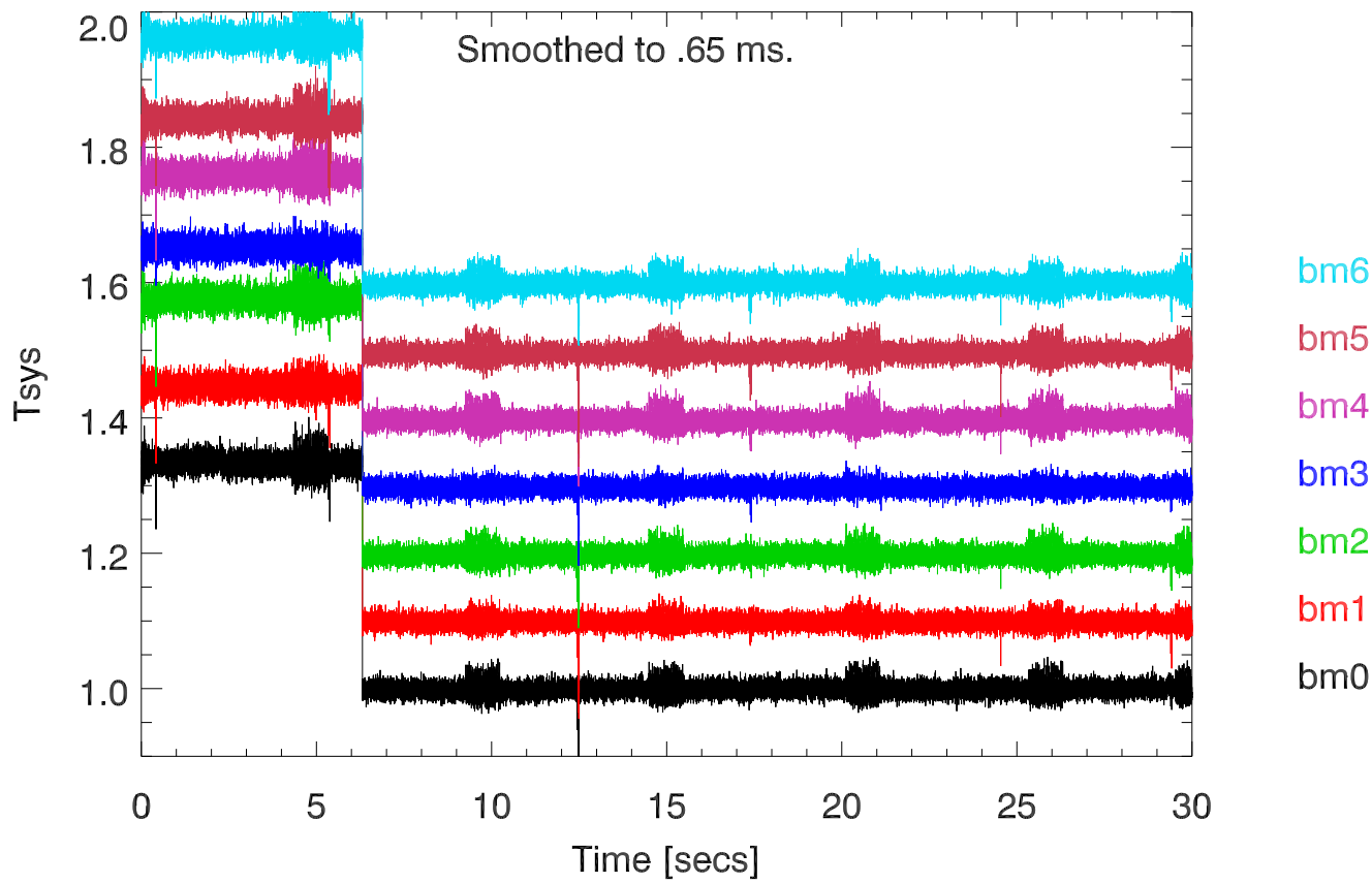
24may12 J1910+1017 TotalPwr(172Mhz) vs Time. 1450Mhz band
