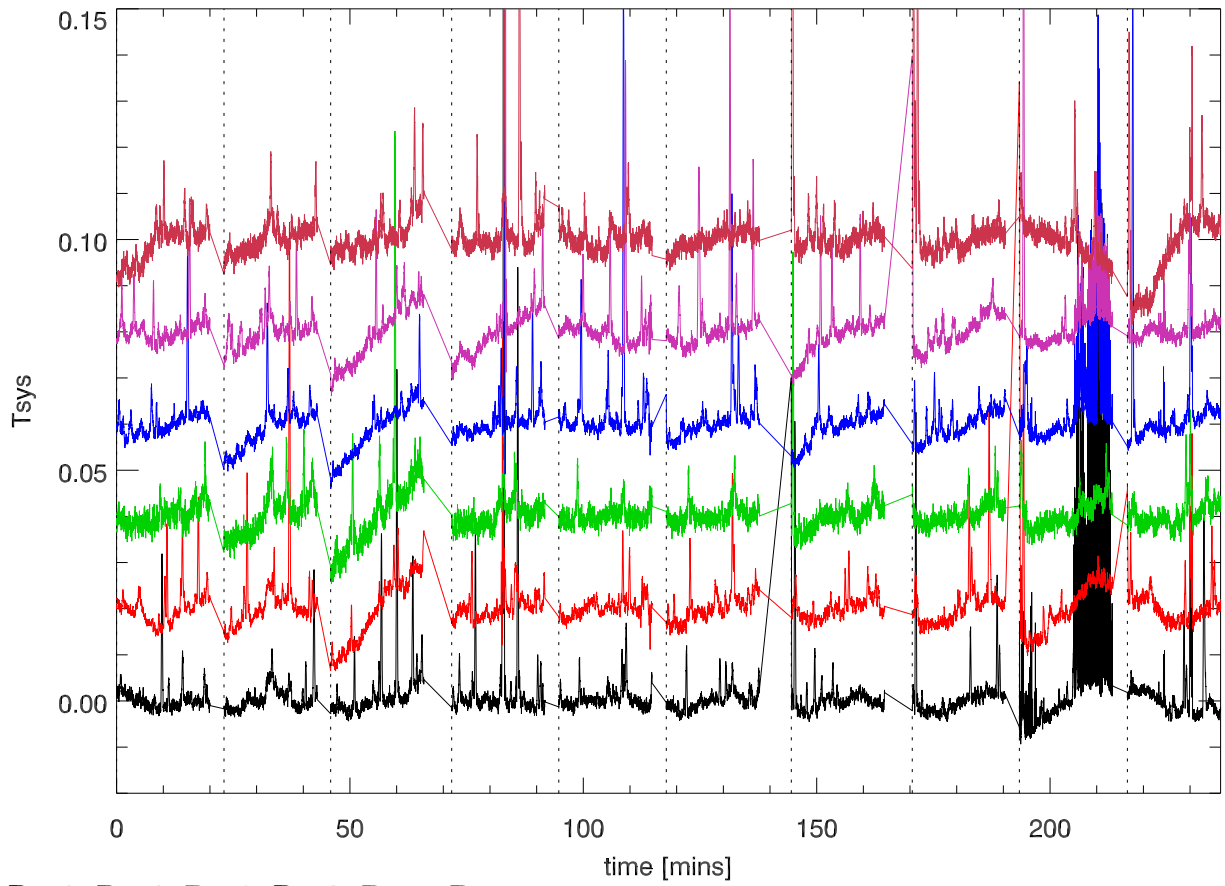
18apr11 alfa a2048 total power vs time. PoIA
