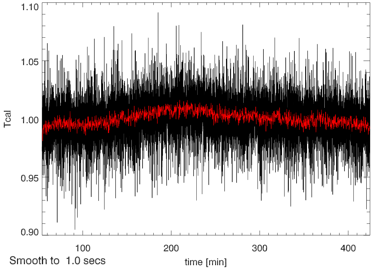
29may12 calOn - calOff Beam6A SigA: 0.026
