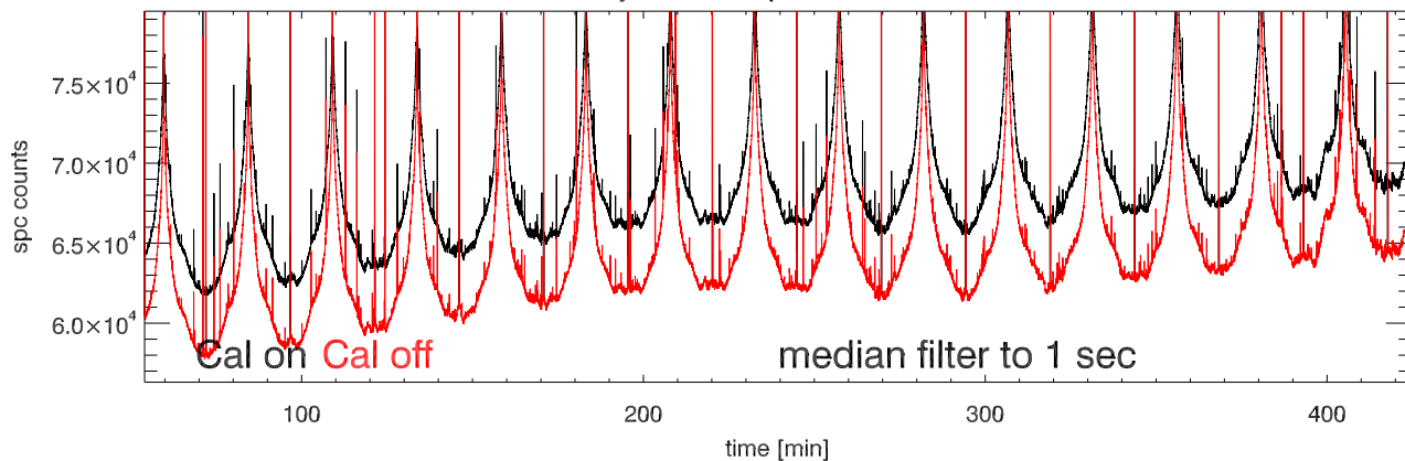
29may12 a2030 tp vs time. Beam6A
