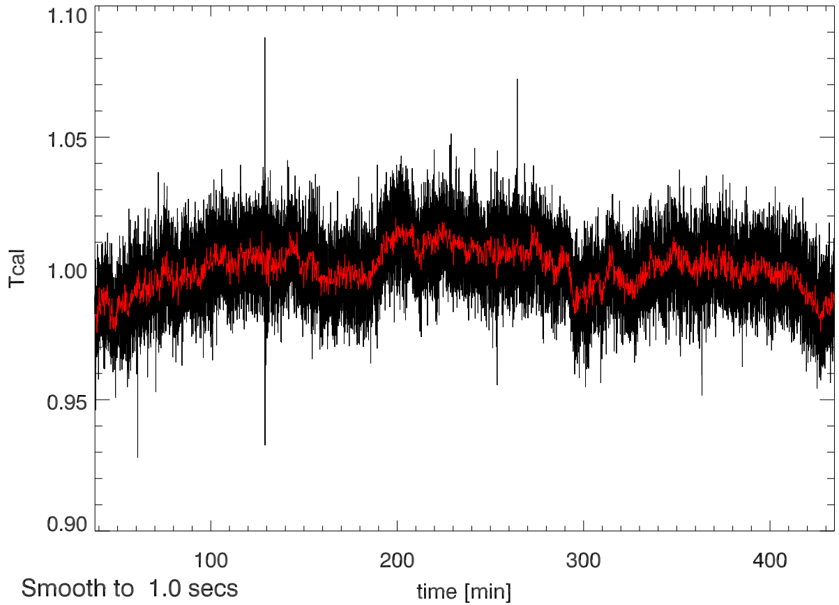
29aug12 calOn - calOff Beam6A SigA: 0.020
