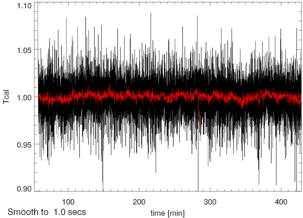
28may12 calOn - calOff Beam6A SigA: 0.025
