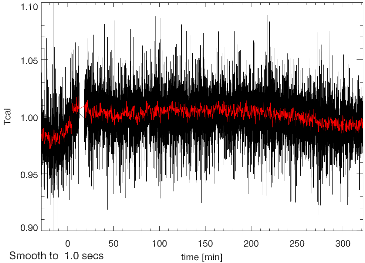
24jun12 calOn - calOff Beam6A SigA: 0.027
