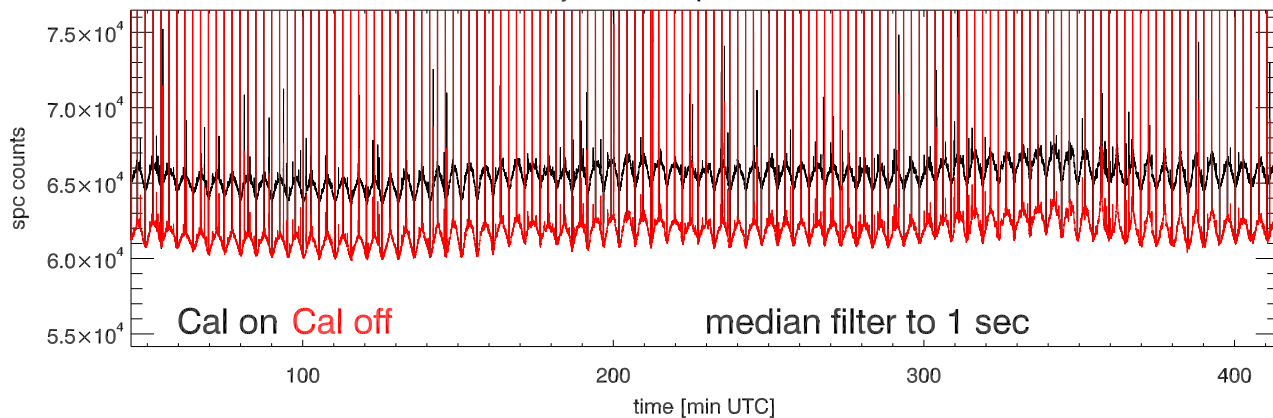
21may13 a2030 tp vs time. Beam6A
