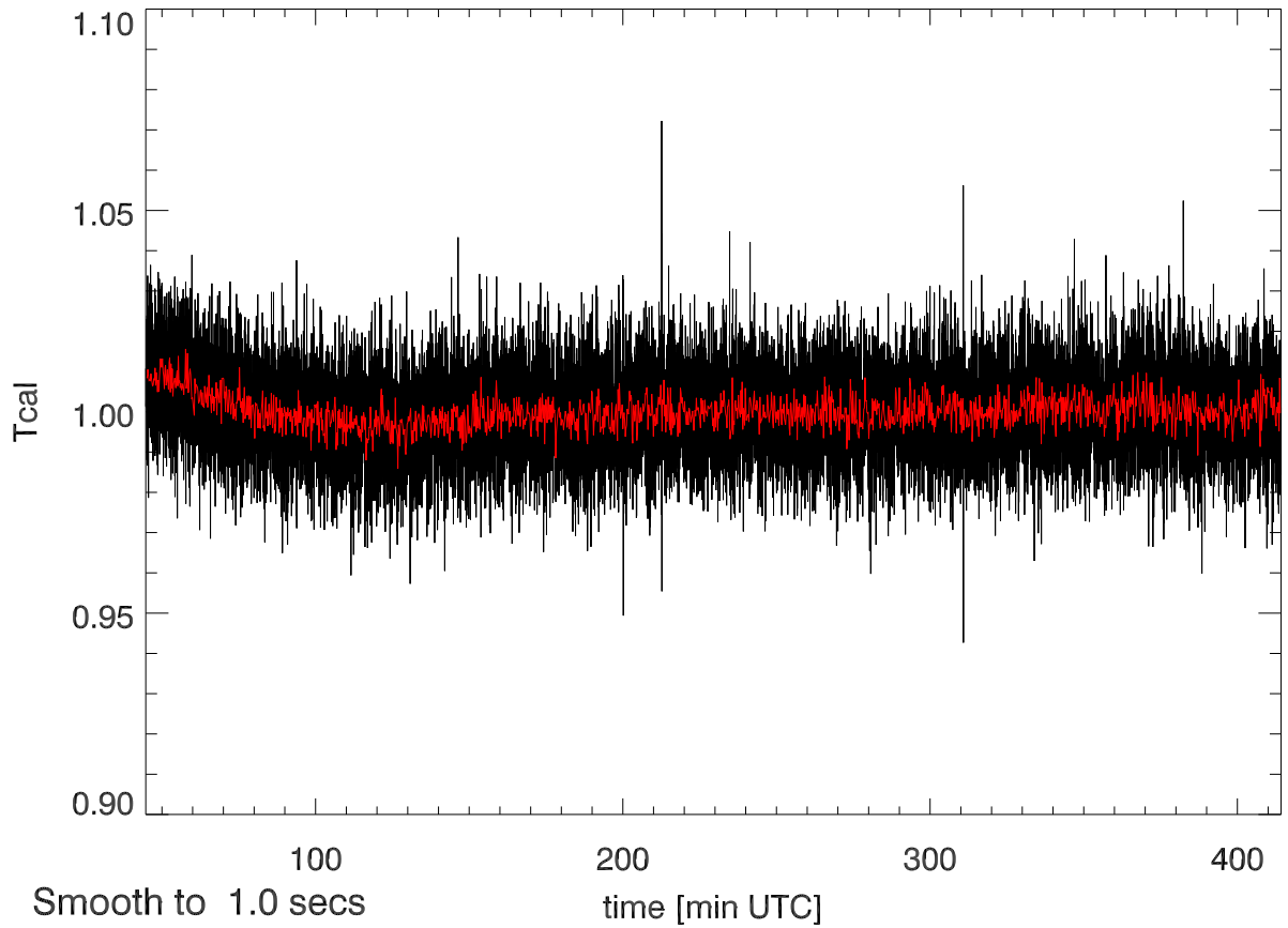
21may13 calOn - calOff Beam6A SigA: 0.019
