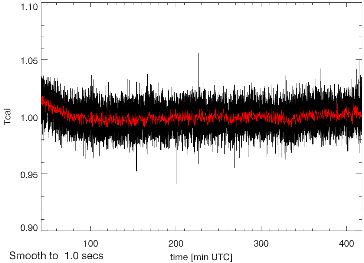
20may13 calOn - calOff Beam6A SigA: 0.019
