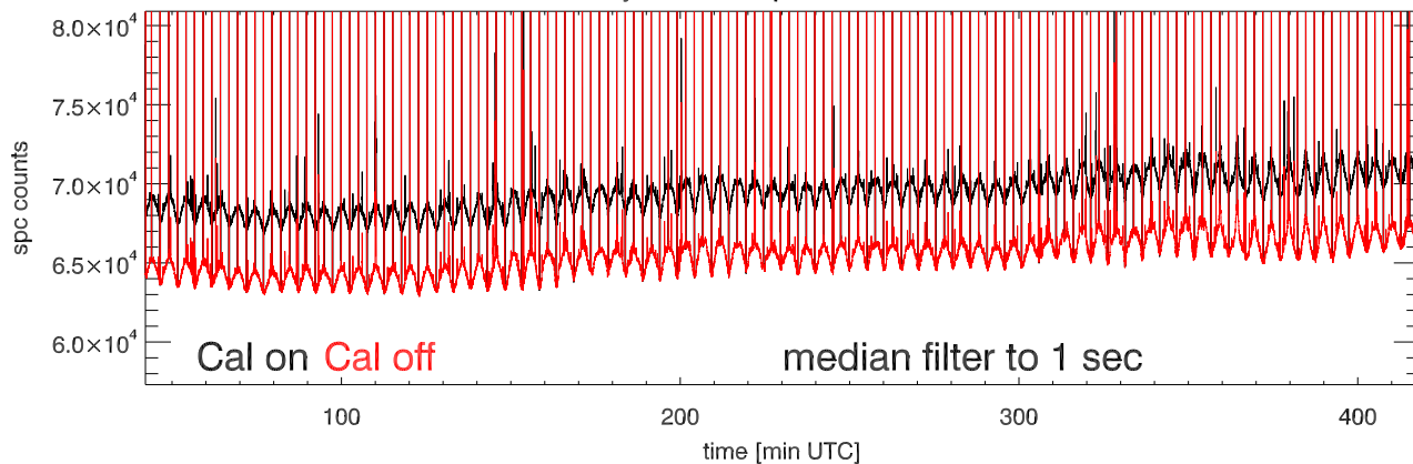
20may13 a2030 tp vs time. Beam6A
