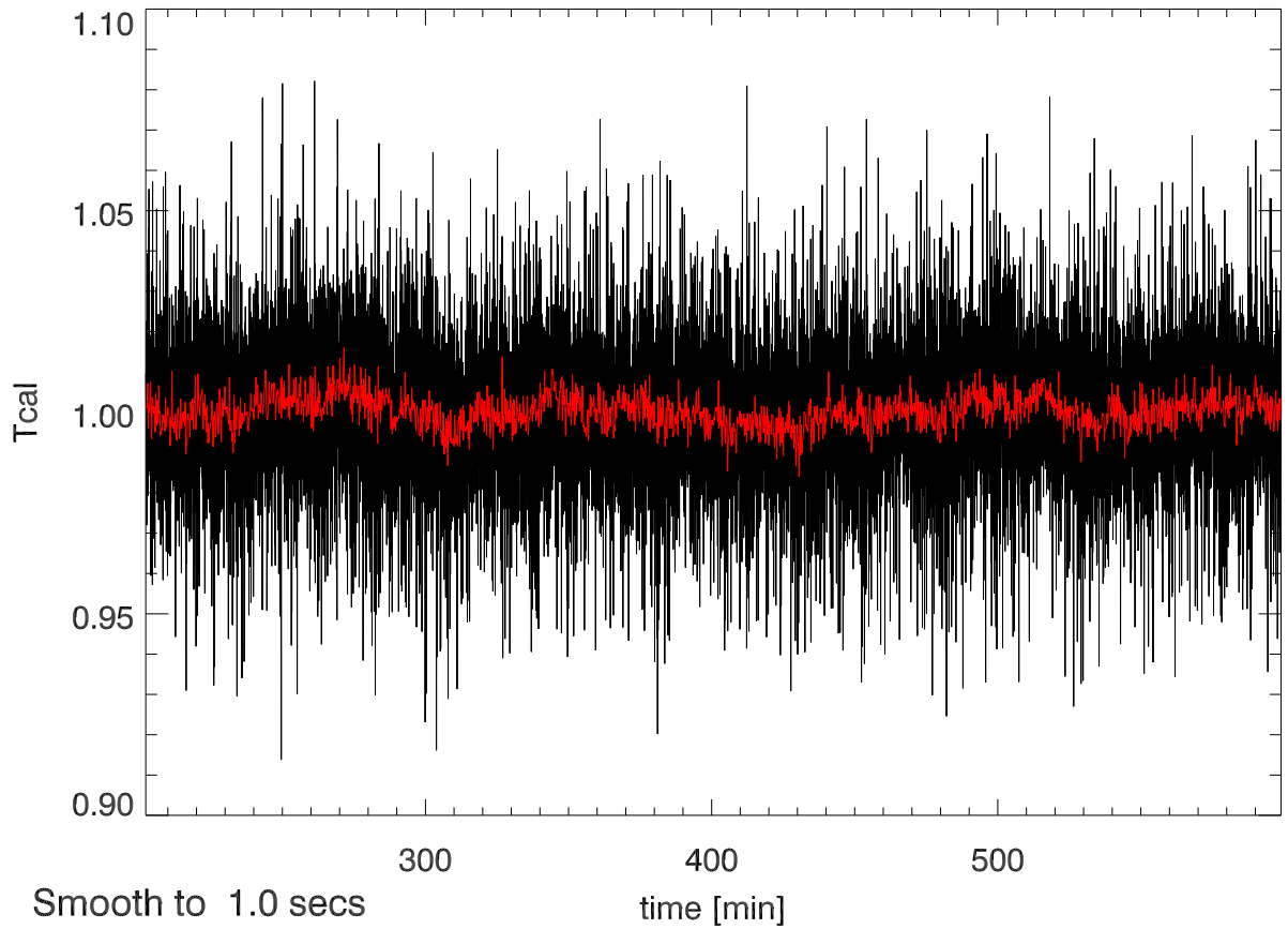
20jul12 calOn - calOff Beam6A SigA: 0.026
