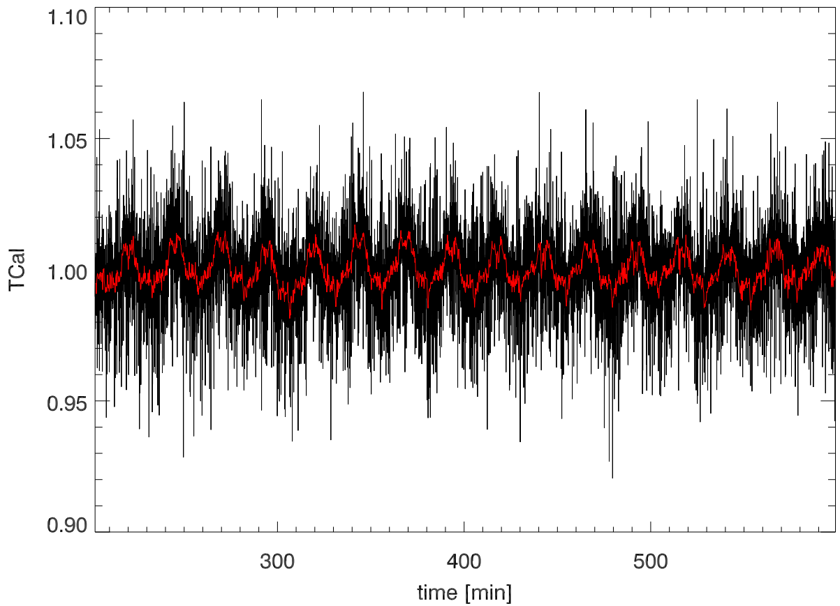
calOn - calOff Beam6B SigB: 0.016
