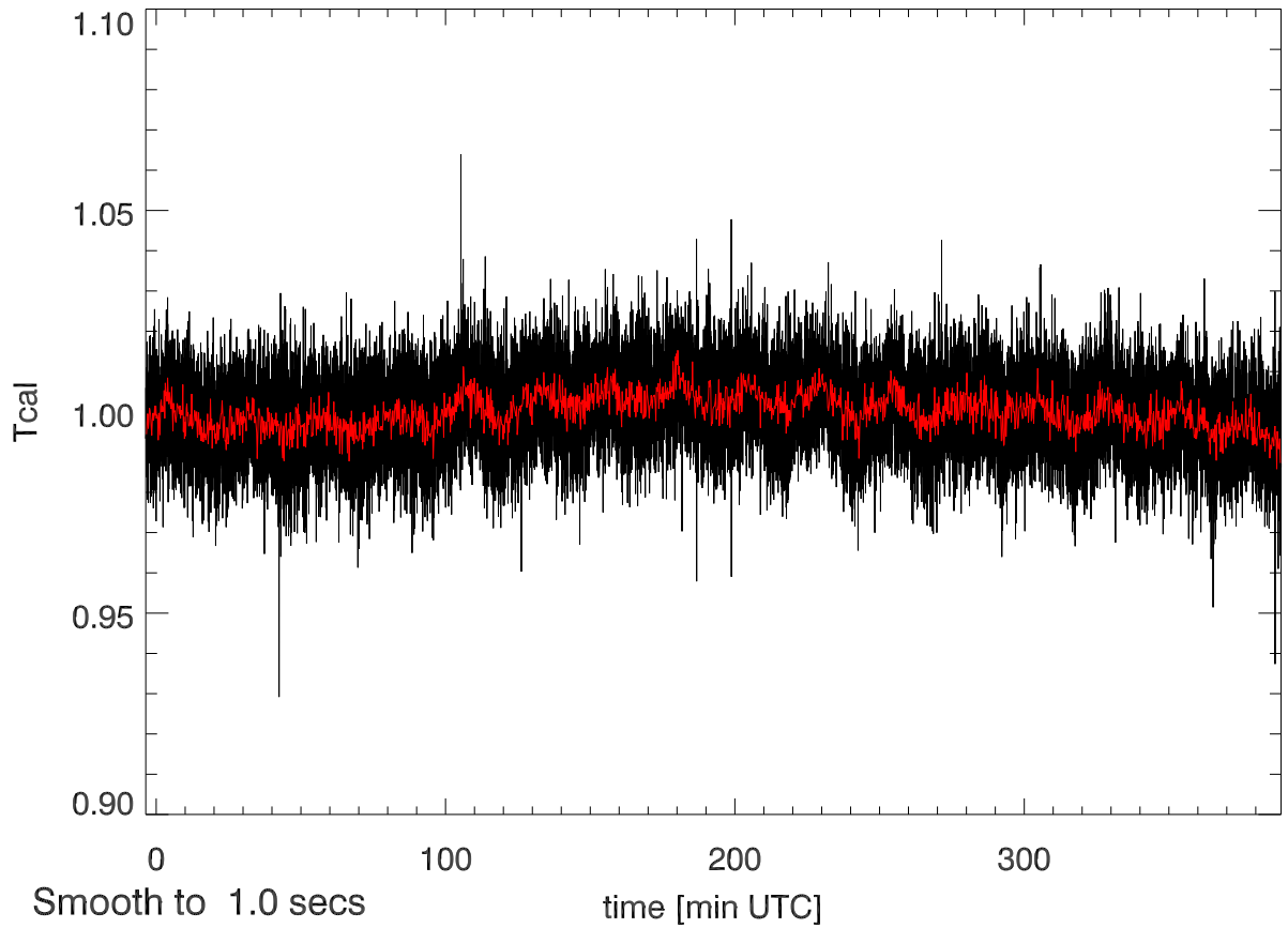
12mar13 calOn - calOff Beam6A SigA: 0.018
