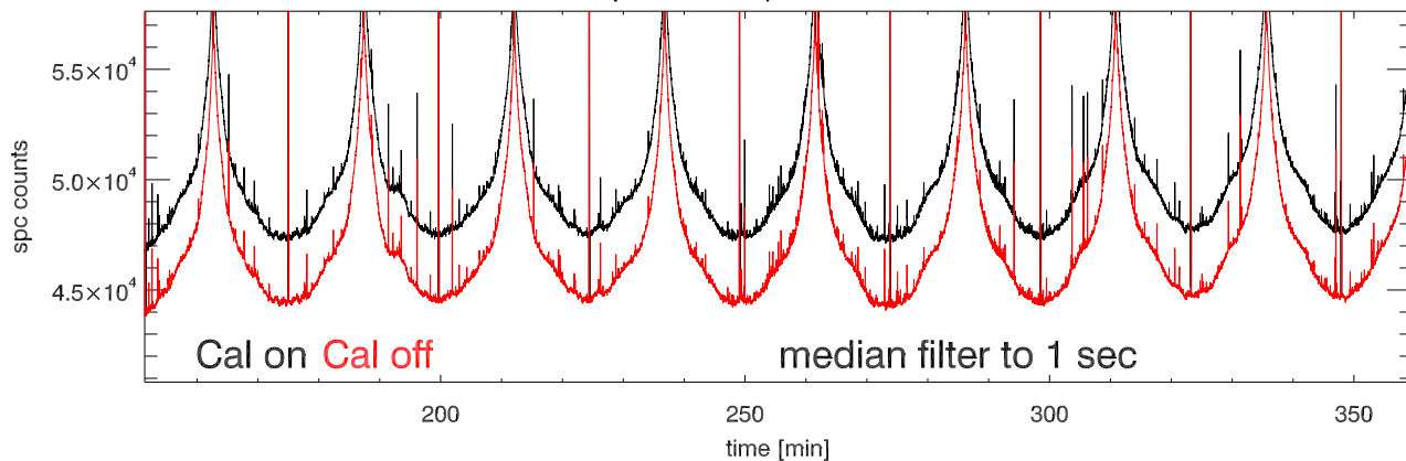
03sep12 a2030 tp vs time. Beam6A
