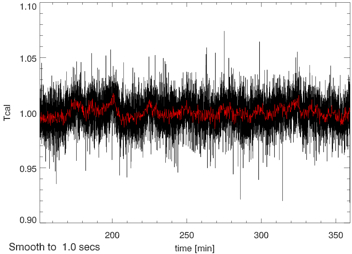
03sep12 calOn - calOff Beam6A SigA: 0.024
