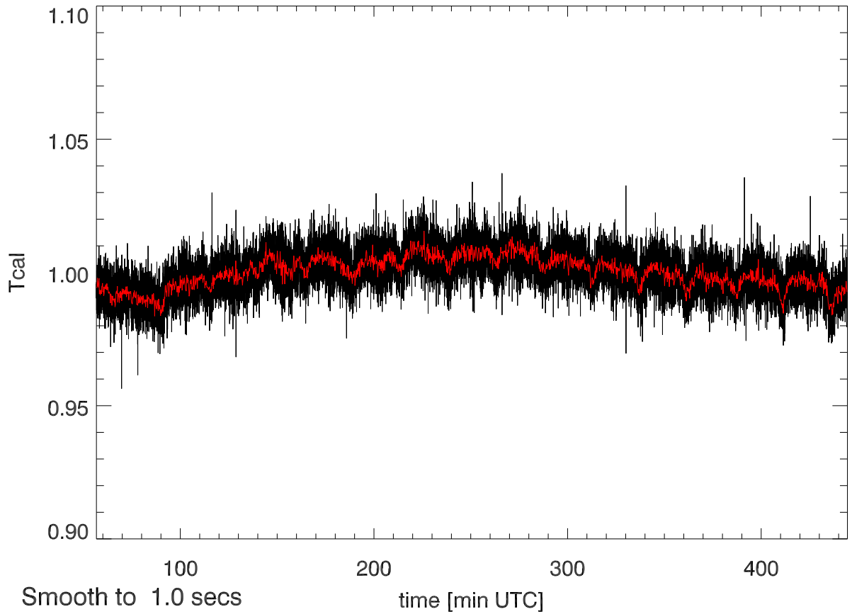
27feb13 calOn - calOff Beam5A SigA: 0.012
