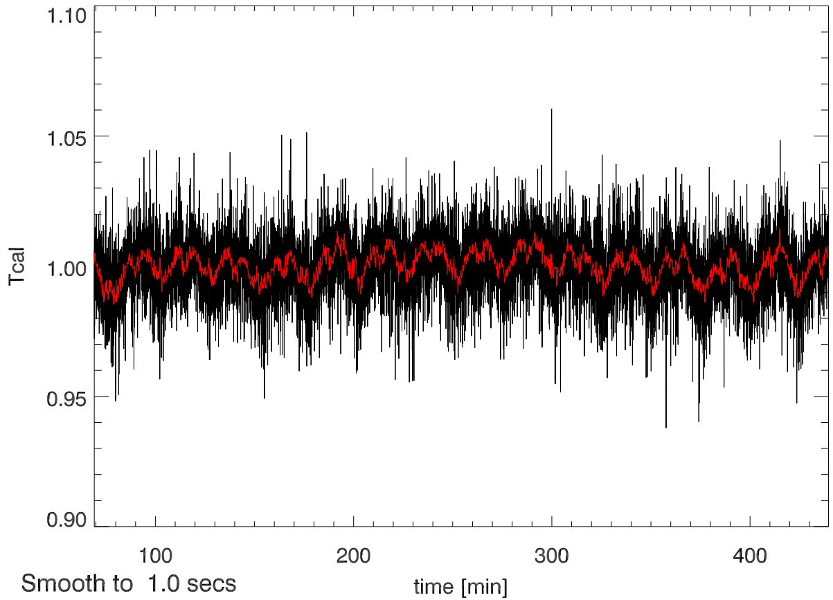
25may12 calOn - calOff Beam5A SigA: 0.016
