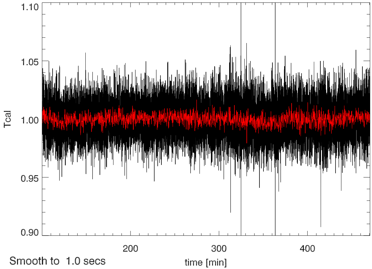
25jun11 calOn - calOff Beam5A SigA: 0.027
