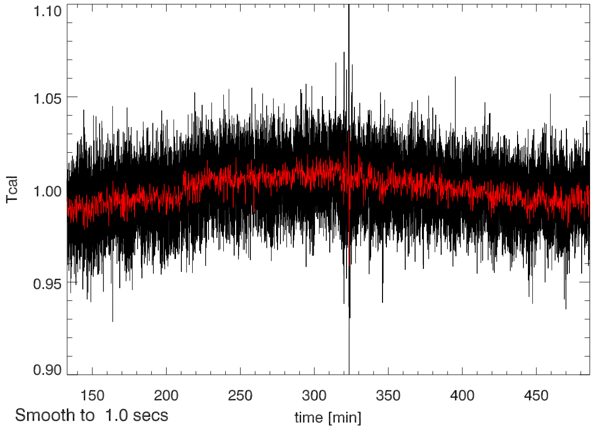
21jun11 calOn - calOff Beam5A SigA: 0.028
