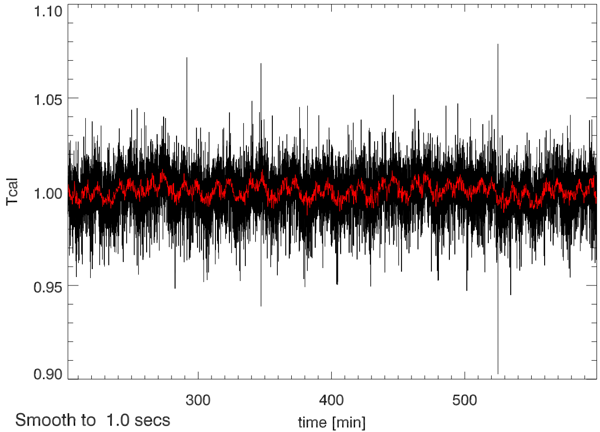
20jul12 calOn - calOff Beam5A SigA: 0.016
