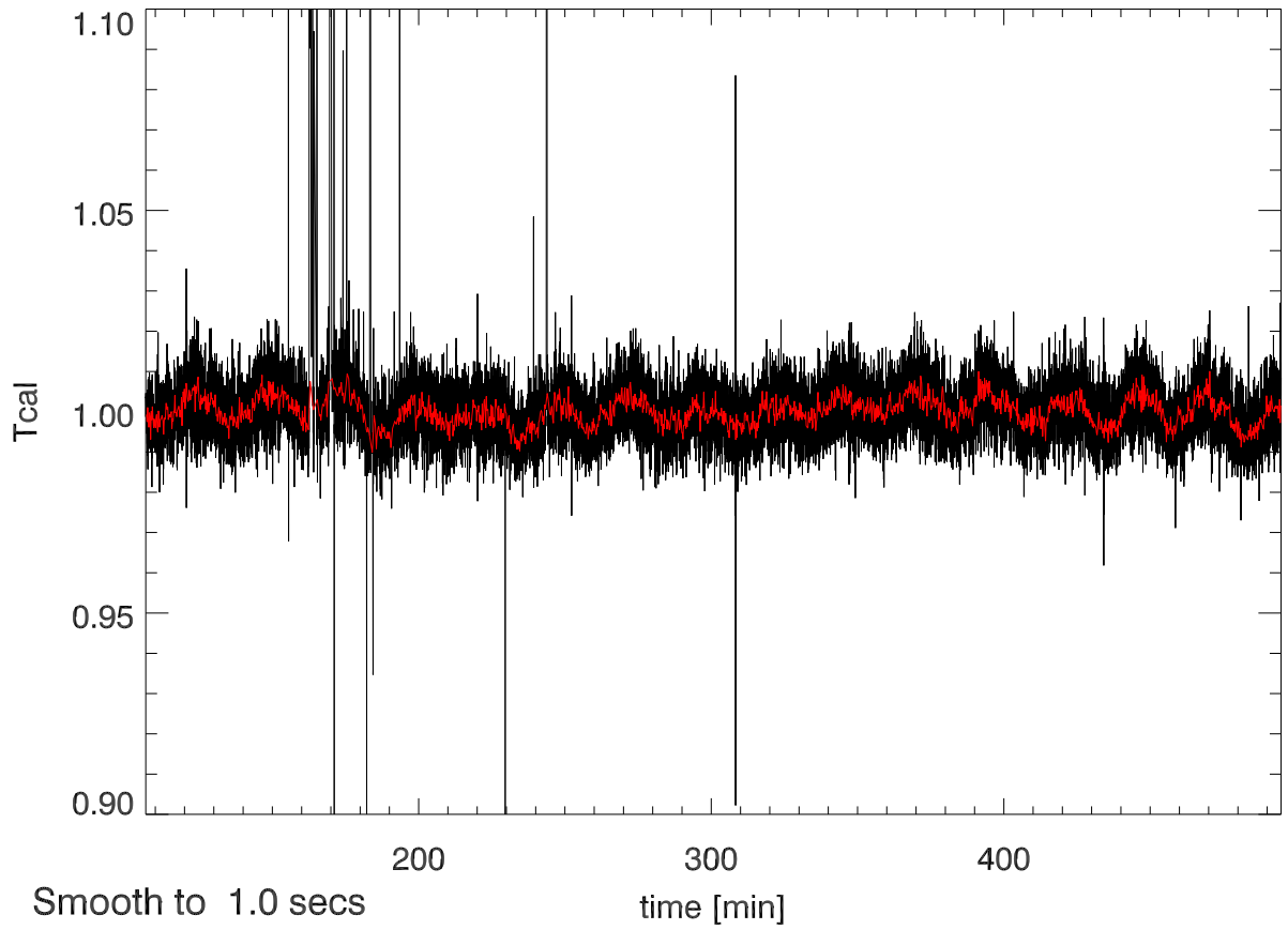
14feb13 calOn - calOff Beam5A SigA: 0.011
