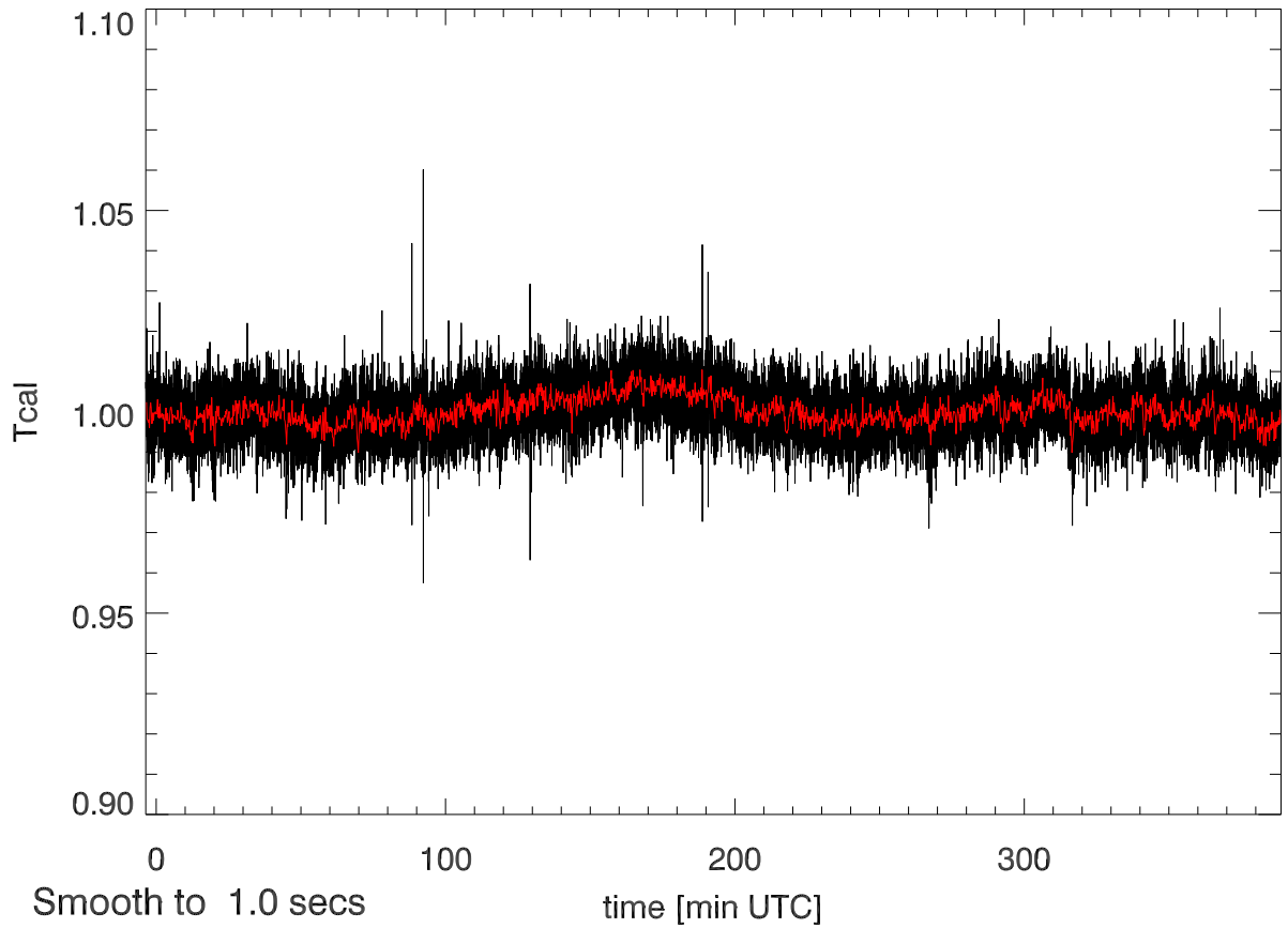
12mar13 calOn - calOff Beam5A SigA: 0.011
