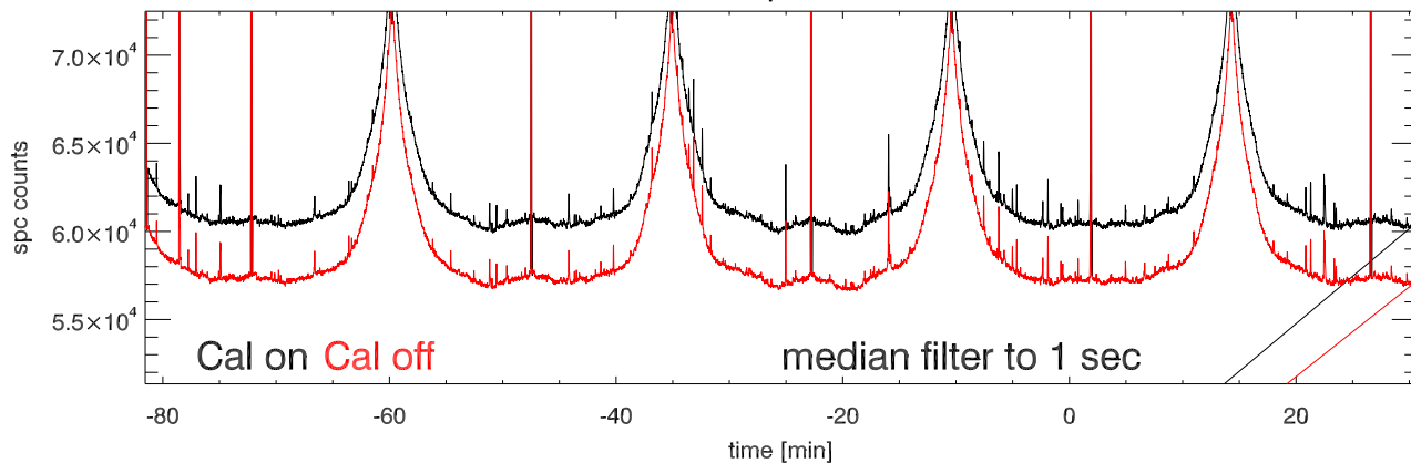
09nov11 a2030 tp vs time. Beam5A
