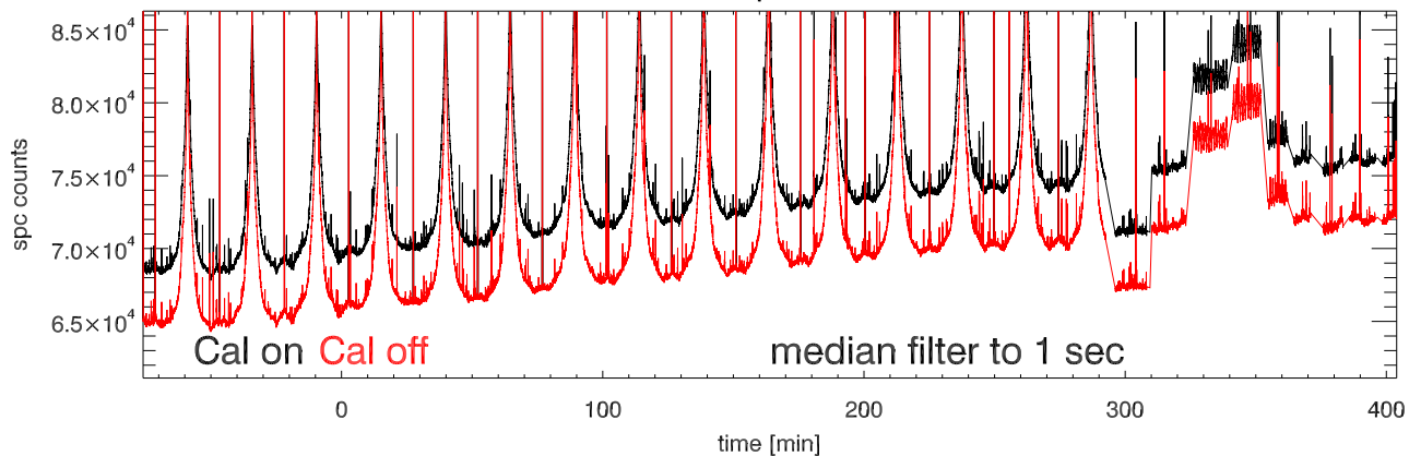
06nov11 a2030 tp vs time. Beam5A
