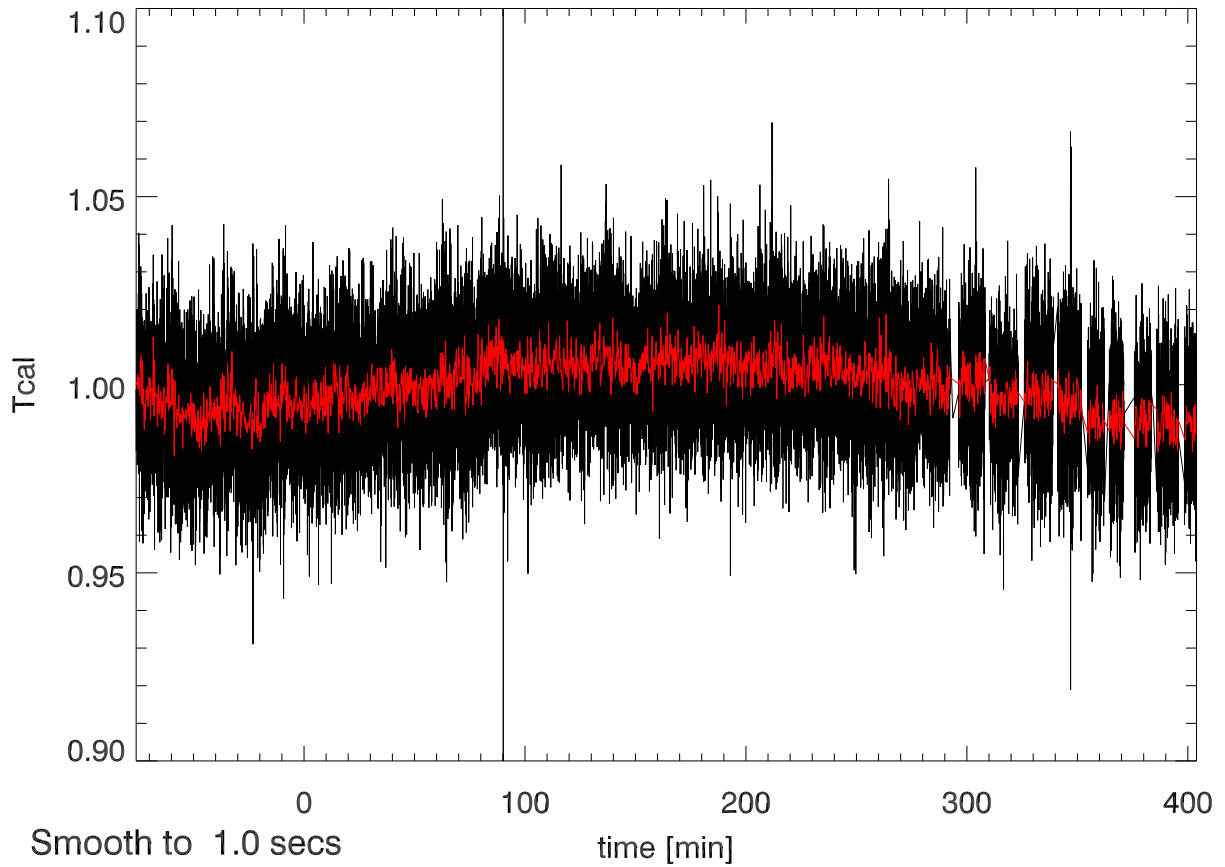
06nov11 calOn - calOff Beam5A SigA: 0.026
