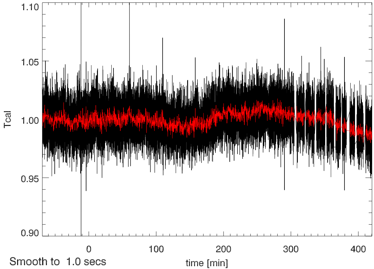
03nov11 calOn - calOff Beam5A SigA: 0.026
