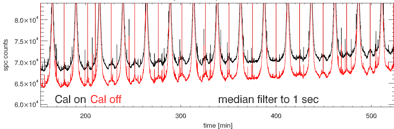
03may12 a2030 tp vs time. Beam5A
