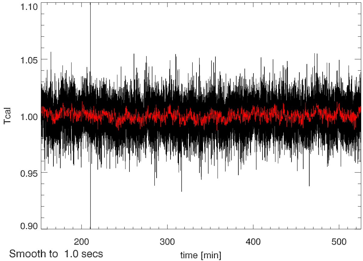
03may12 calOn - calOff Beam5A SigA: 0.025
