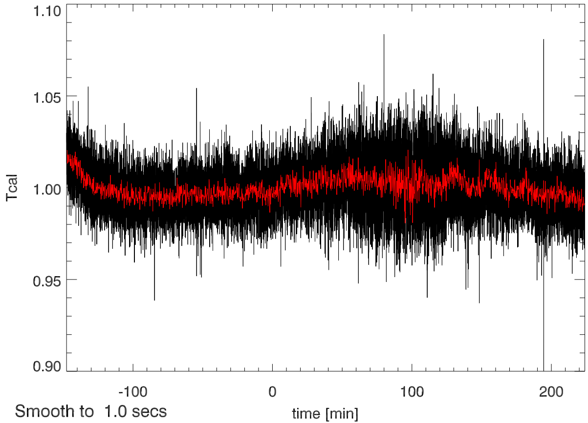
23nov11 calOn - calOff Beam4A SigA: 0.024
