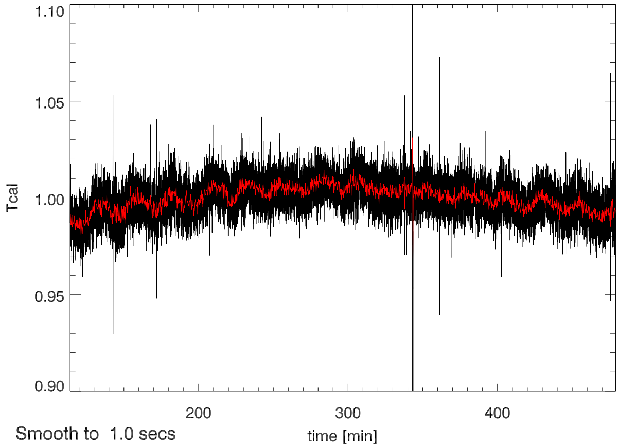
23jun11 calOn - calOff Beam4A SigA: 0.015
