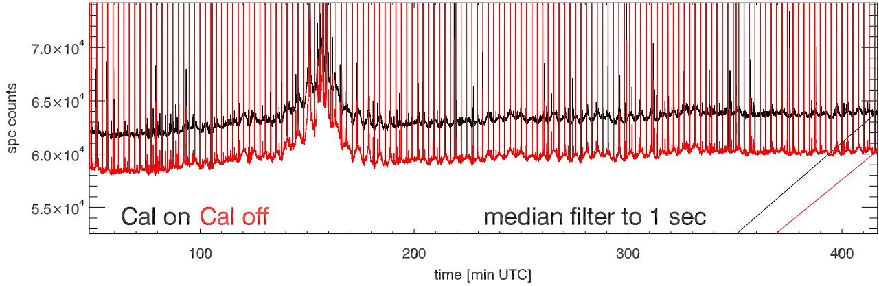
21aug13 a2030 tp vs time. Beam4A
