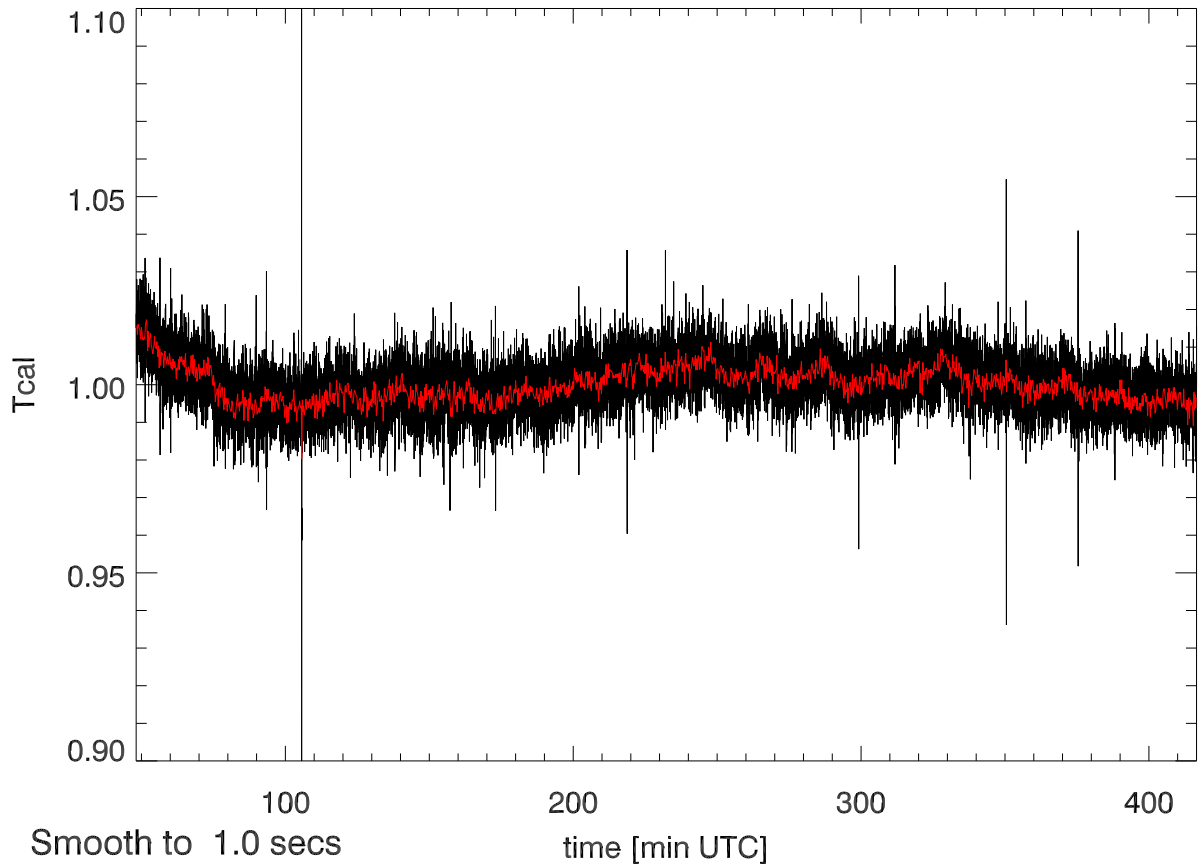
21aug13 calOn - calOff Beam4A SigA: 0.011
