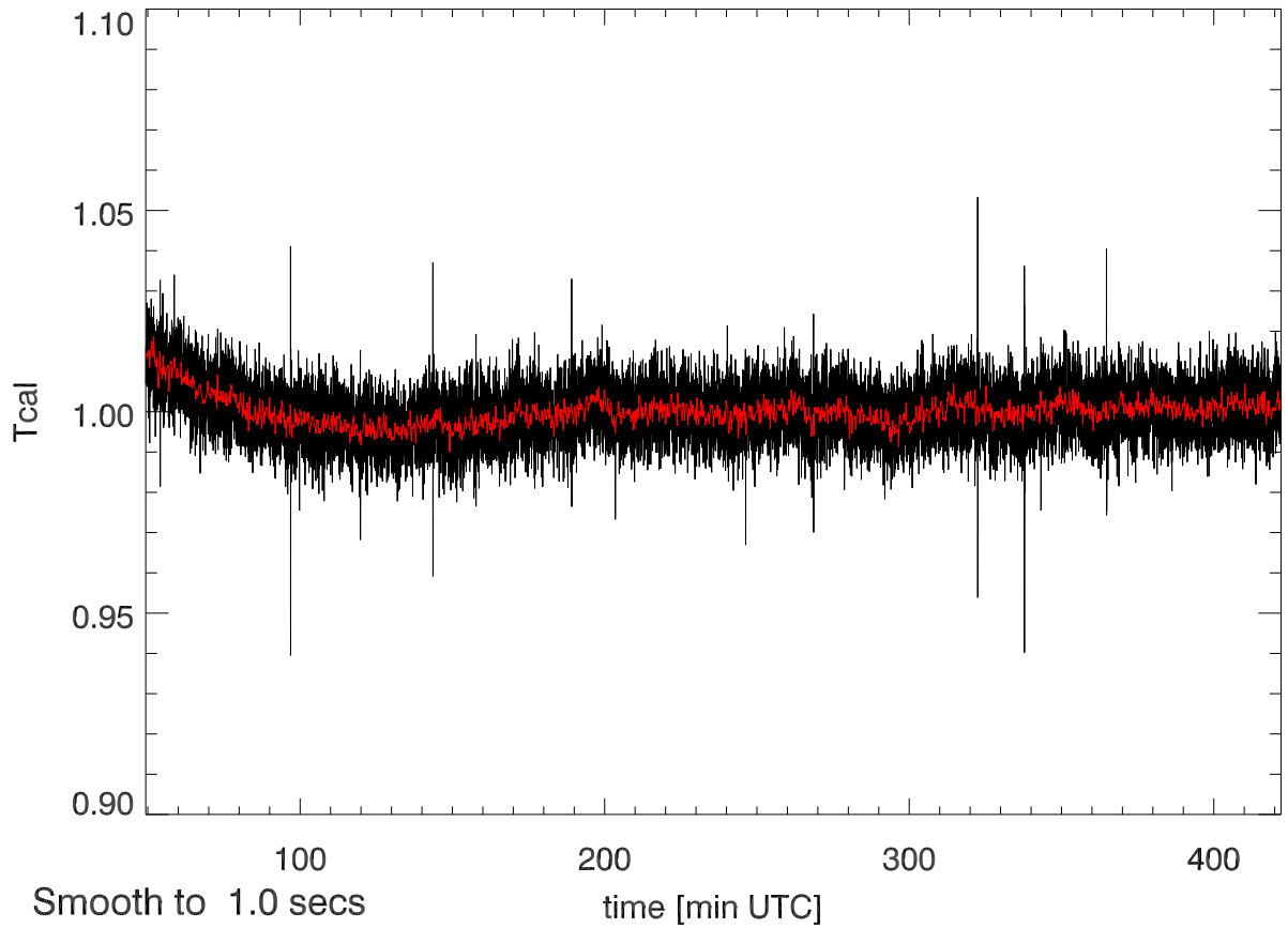
19may13 calOn - calOff Beam4A SigA: 0.011
