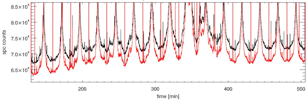
calOn - calOff Beam4A
