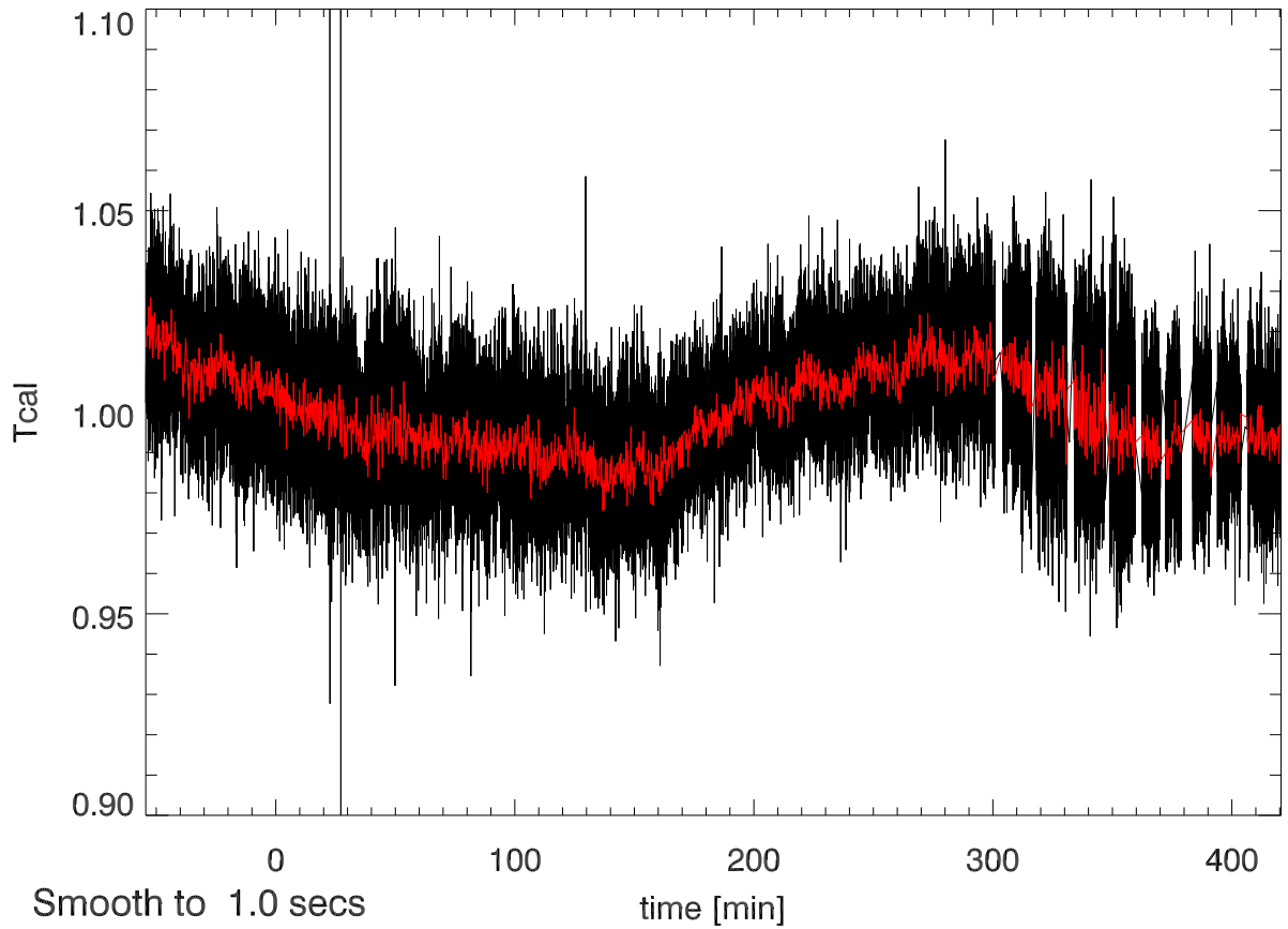
04nov11 calOn - calOff Beam4A SigA: 0.026
