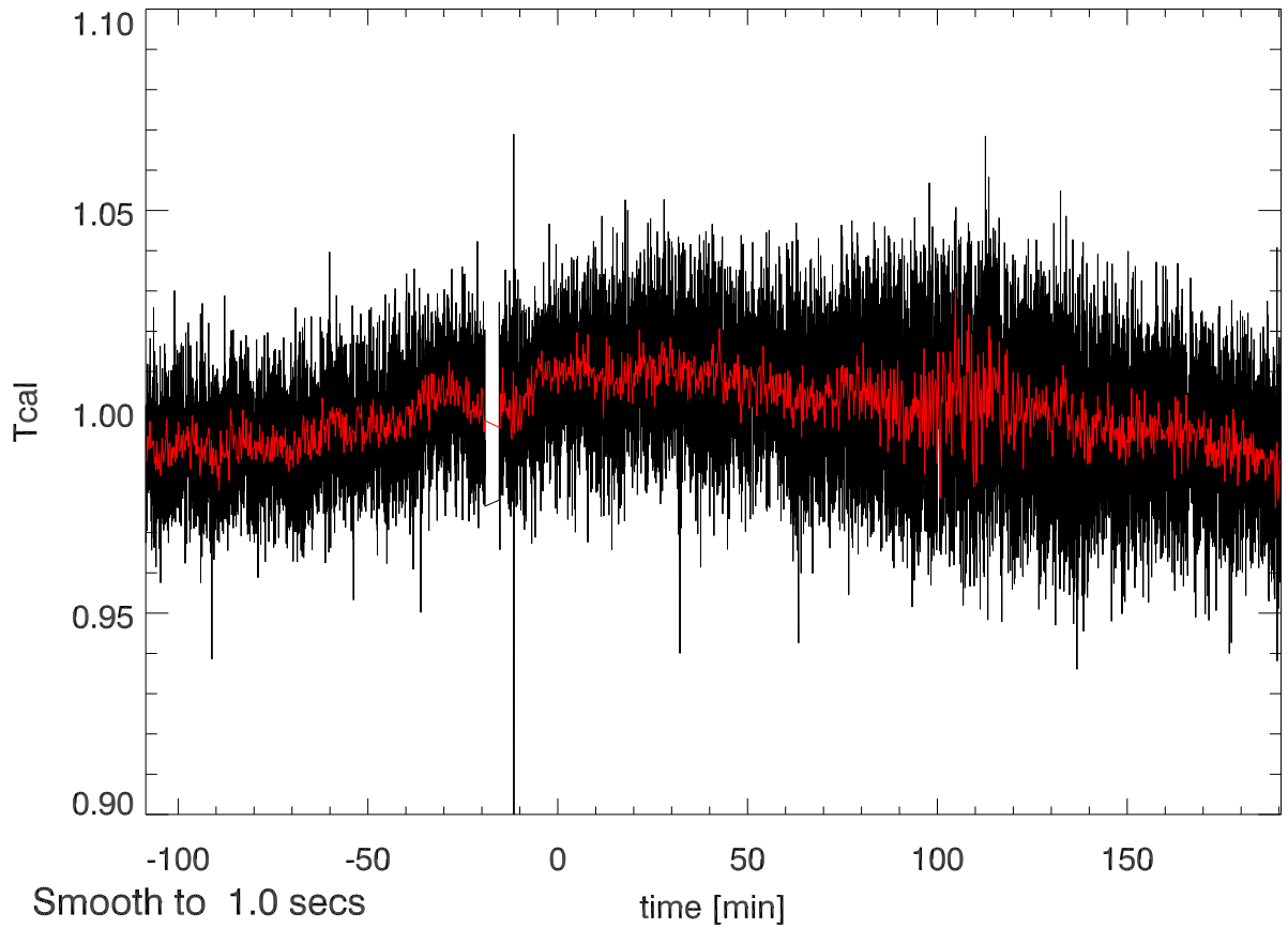
02dec11 calOn - calOff Beam4A SigA: 0.026
