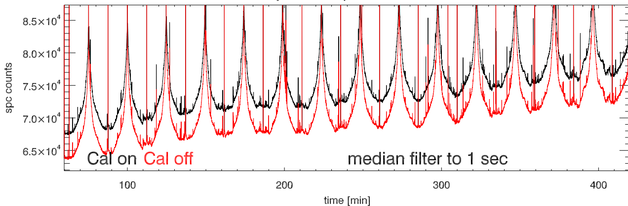
30may12 a2030 tp vs time. Beam3A
