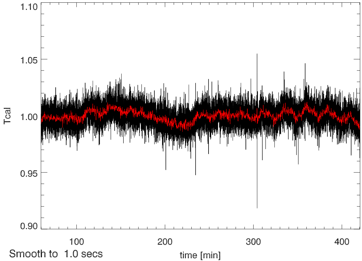
30may12 calOn - calOff Beam3A SigA: 0.015
