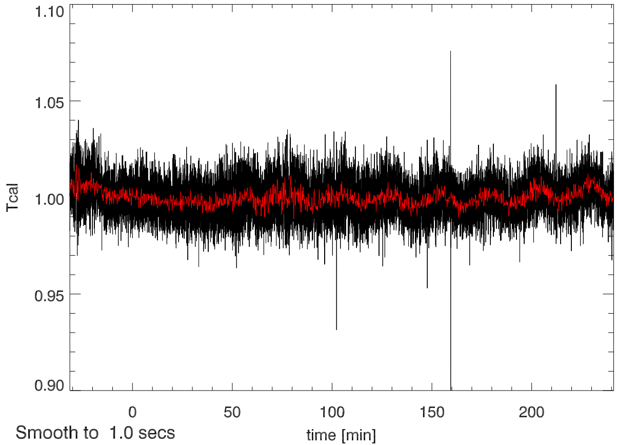
23may11 calOn - calOff Beam3A SigA: 0.016
