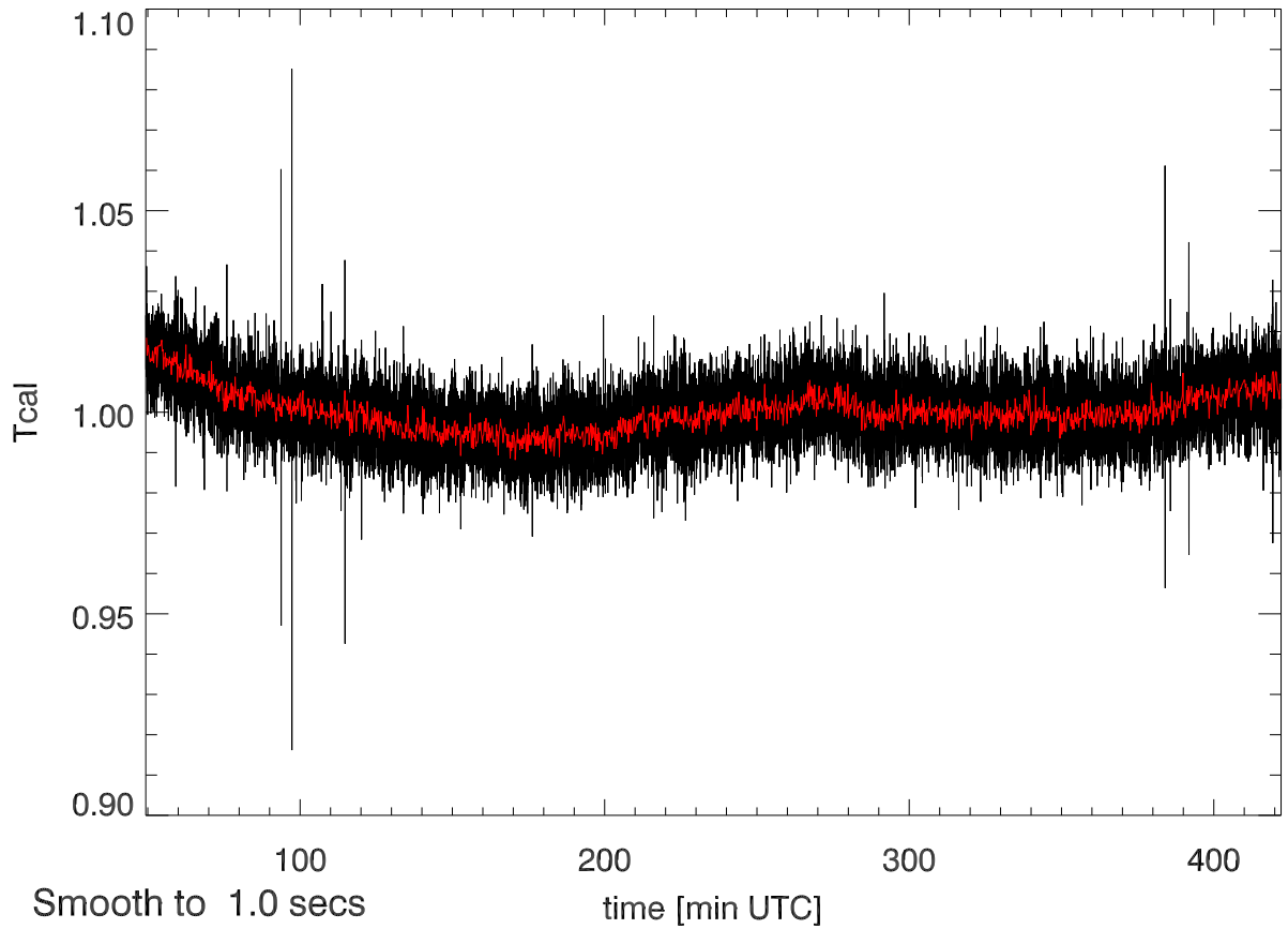
19may13 calOn - calOff Beam3A SigA: 0.013
